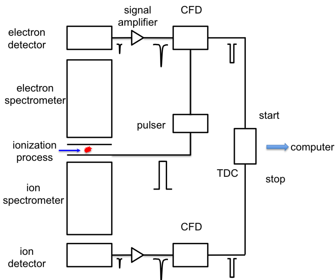
Figure 1. Schematics of a PEPICO experimental setup (see text for details). Ions and electrons produce electric signals in the respective detectors, typically a secondary electron multiplier (channeltron or microchannel plate). CFD: Constant Fraction Discriminator, which converts detector pulses into norm pulses with a stable timing, TDC: Time to digital converter.
