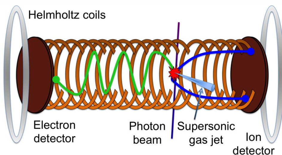
Figure 5. Schematics of a COLTRIMS experiment (see text for details).
