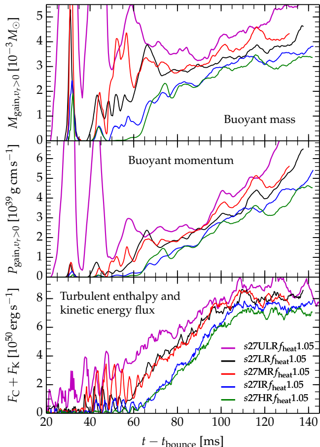
Figure 11. Comparison of buoyant mass (top panel), buoyant momentum (center panel), and radial convective enthalpy and kinetic energy fluxes (bottom panel, cf. Equation 10) for simulations with five different resolutions of the strong neutrino heating case. Higher-resolution simulations, in particular in the first \sim 100 ms after bounce (before shock expansion sets in), have smaller M_{\text{gain}, v_r > 0} , P_{\text{gain}, v_r > 0} , and F_C + F_K than lower resolution simulations.
