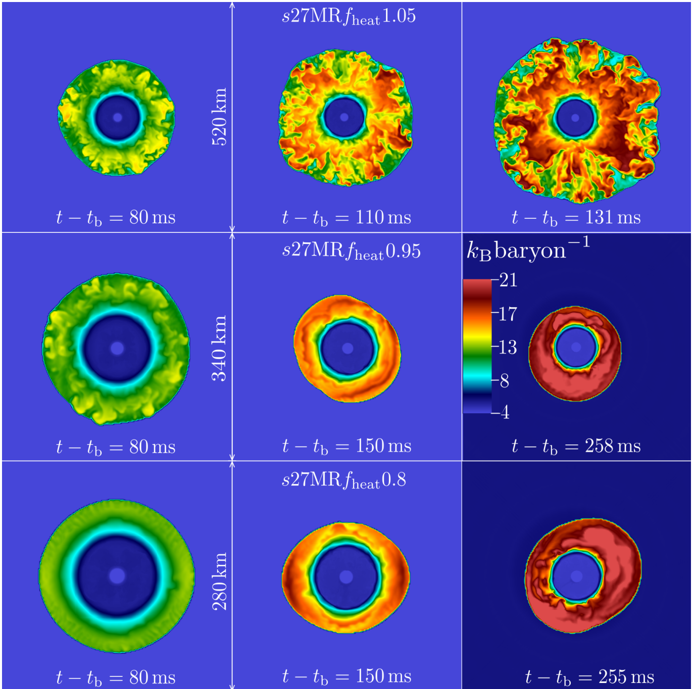
Figure 4. Colormaps of specific entropy in the x - z plane in models s27MR_{f_{\text{heat}} 1.05} (strong neutrino heating; top row), s27MR_{f_{\text{heat}} 0.95} (moderate neutrino heating; center row), and s27MR_{f_{\text{heat}} 0.8} (weak neutrino heating; bottom row) at a range of postbounce times. Note that the scale of the region shown is different for each model. Model s27MR_{f_{\text{heat}} 1.05} is dominated by neutrino-driven convection. Model s27MR_{f_{\text{heat}} 0.95} shows neutrino-driven convection at early times, but subsequently shows signs of coherent shock dynamics typical for the SASI. Model s27MR_{f_{\text{heat}} 0.8} never develops significant neutrino-driven convection and becomes dominated by the SASI.
