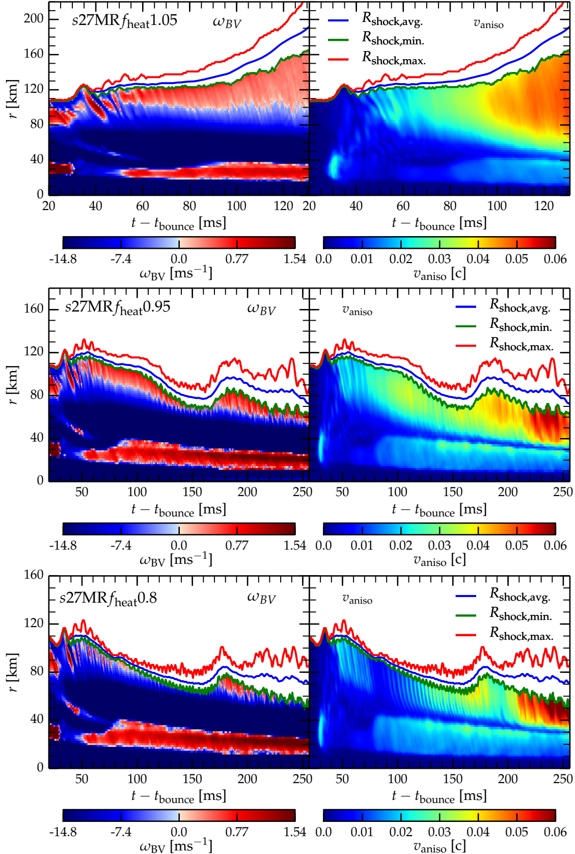
Figure 7. Colormaps showing radial slices of the angle-averaged Brunt-Väisälä (BV) frequency \omega_{BV} (Equation 5; left panels) and anisotropic velocity v_{\text{aniso}} (Equation 7; right panels) in models s27MR f_{\text{heat}} 1.05 (top panels), s27MR f_{\text{heat}} 0.95 (center panels), and s27MR f_{\text{heat}} 0.8 (bottom panels). Also shown are the maximum (red curves), the average (blue curves), and the minimum (green curves) shock radii. We do not show \omega_{BV} and v_{\text{aniso}} outside the minimum shock radius. Note the differing temporal and radial scales chosen for different models.
