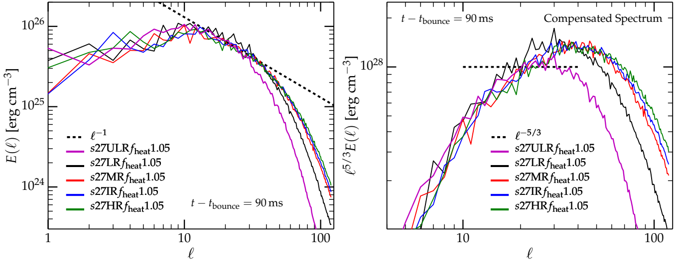
Figure 12. Left panel: Angular spectra of the turbulent kinetic energy density for five different resolutions at 90ms after bounce in the strong neutrino heating case. The turbulent transport of energy to small scales becomes increasingly efficient with increasing resolution. Decreasing resolution leads to an onset of strong dissipation at smaller \ell . Right panel: Compensated ( \ell^{5/3} rescaled) turbulent spectra. The dashed line indicates the range in \ell where we expect the inertial range and where the spectrum should be flat if E(\ell) \propto \ell^{-5/3} were realized as predicted by theory.
