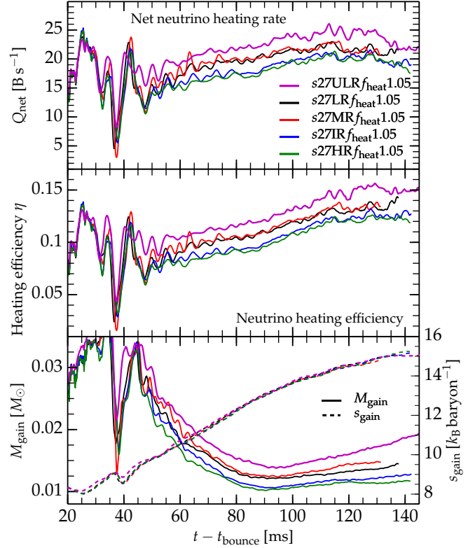
Figure 10. Time evolution of the net neutrino heating Q_{\text{net}} (top panel), heating efficiency \eta (center panel), mass in the gain region M_{\text{gain}} (bottom panel, left ordinate), and the average entropy in the gain region s_{\text{gain}} (bottom panel, right ordinate) for the case of strong neutrino heating and five different resolutions. Low resolution results in artificially efficient neutrino heating and in an overestimate of the mass in the gain region.
