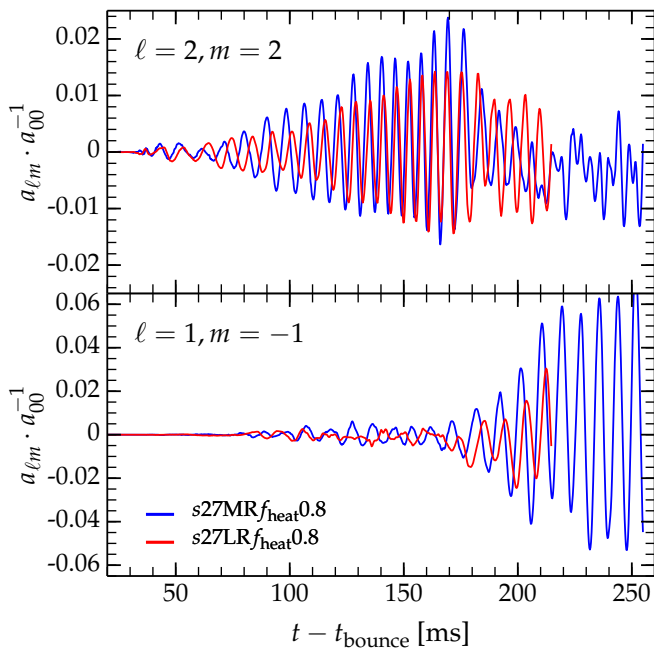
Figure 14. Comparison of select normalized mode amplitudes a_{\ell m} \cdot a_{00}^{-1} of the shock front between the LR and MR simulations of the SASI dominated f_{\text{heat}} = 0.8 model. The top panel shows the \ell = 2, m = 2 mode and the bottom panel shows the \ell = 1, m = -1 mode. The qualitative evolution of the modes are nearly independent of resolution and behave as discussed in §4.2 for this model. However, the magnitude of the mode amplitudes is generally lower in the lower-resolution simulation. The resolutions differ by \sim 30\% .
