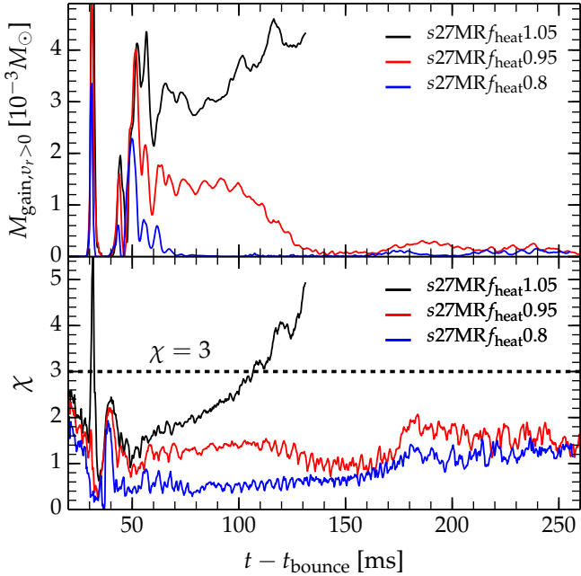
Figure 3. Top panel: The mass M_{\text{gain}, v_r > 0} in the gain region with positive radial velocity (“buoyant mass”) in models s27MR_{f_{\text{heat}}1.05} (strong neutrino heating), s27MR_{f_{\text{heat}}0.95} (moderate neutrino heating), and s27MR_{f_{\text{heat}}0.8} (weak neutrino heating). Bottom panel: The Foglizzo \chi parameter (cf. Equation 6) as a function of postbounce time for the three models. The horizontal line at \chi = 3 marks the point where convection is expected to develop in the gain region. We calculate \chi on the basis of angle-averaged, but not time-averaged quantities.
