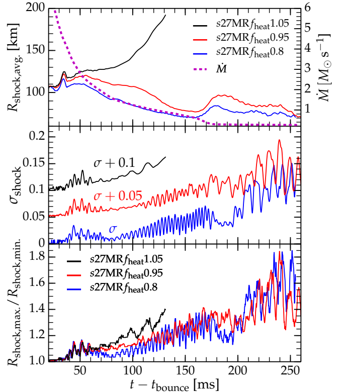
Figure 1. Top panel: Average shock radius evolution for models with strong ( s27MRf_{\text{heat}}1.05 ), medium ( s27MRf_{\text{heat}}0.95 ), and weak ( s27MRf_{\text{heat}}0.8 ) neutrino heating. Model s27MRf_{\text{heat}}1.05 , due to its strong neutrino heating, shows the onset of an explosion already \sim 100 ms after bounce. The models with moderate and weak neutrino heating fail to show signs of explosion, but exhibit a transient shock expansion when the accretion rate ( \dot{M} , dashed magenta line) drops at the time the silicon interface accretes through the stalled shock. Center panel: Normalized root mean square deviation \sigma_{\text{shock}} of the shock radius from its angle averaged value. Bottom panel: Ratio of the maximum shock radius to the minimum shock radius. The models with moderate and weak neutrino heating exhibit strong periodic oscillations in the shock radius ratio and in \sigma_{\text{shock}} . These variations are the tell-tale signs of SASI activity in these models.
