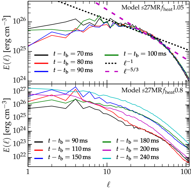
Figure 8. Top panel: Angular spectra E(\ell) of the angular kinetic energy density of convective turbulent motion (Equation 9) in model s27MR_{f_{\text{heat}}1.05} at a range of postbounce times before the onset of shock expansion. We overplot lines indicating \ell^{-5/3} (Kolmogorov) and \ell^{-1} scaling. The energy containing range is near \ell = 5 - 10 and should be linked by the inertial range to the dissipation scale at large \ell . E(\ell) is most consistent with \ell^{-1} scaling in the “inertial range,” which suggests that numerical viscosity affects the efficiency of kinetic energy from large to small scales. Bottom panel: Angular spectra E(\ell) for model s27MR_{f_{\text{heat}}0.8} (weak neutrino heating) at various postbounce times. In this SASI-dominated model, turbulence is driven by shear and entropy gradients associated with secondary shocks. The E(\ell) spectrum is highly nonstationary at all \ell .
