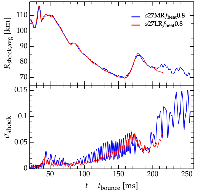
Figure 13. Top panel: Comparison of the average shock radius evolution in the MR and LR simulations of the SASI dominated f_{\text{heat}} = 0.8 model with weak neutrino heating. The MR and LR resolutions differ by \sim 30\% . The shock radius evolution is almost independent of resolution in this model and until \sim 200 ms after bounce. Then, the shock in the higher-resolution (MR) simulations expands somewhat, possibly related to the appearance of large-scale \ell = 1 SASI modes at this time (cf. Figure 14). Bottom panel: The normalized root mean square deviation \sigma_{\text{shock}} of the shock radius from its angle averaged value in the MR and LR simulations. The oscillations in \sigma_{\text{shock}} , which are due to the SASI, are much stronger in the MR simulation, indicating that the SASI is weaker in the LR simulation (cf. Figure 14).
