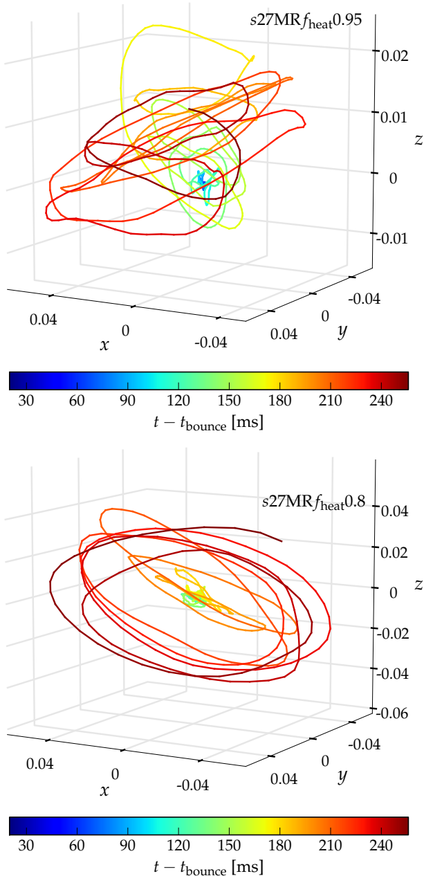
Figure 6. Evolution of the normalized \ell = 1 mode vector \mathbf{a}_1/a_{00} for models s27MR_{f_{\text{heat}}0.95} (top panel) and s27MR_{f_{\text{heat}}0.8} (bottom panel). The viewing directions on each panel are chosen to be perpendicular to the plane of the spiral SASI motion when it reaches the largest amplitude. The color of the graphs demark time. Both models exhibit spiral SASI oscillations, but they are strongest in the model with weakest neutrino heating, s27MR_{f_{\text{heat}}0.8} .
