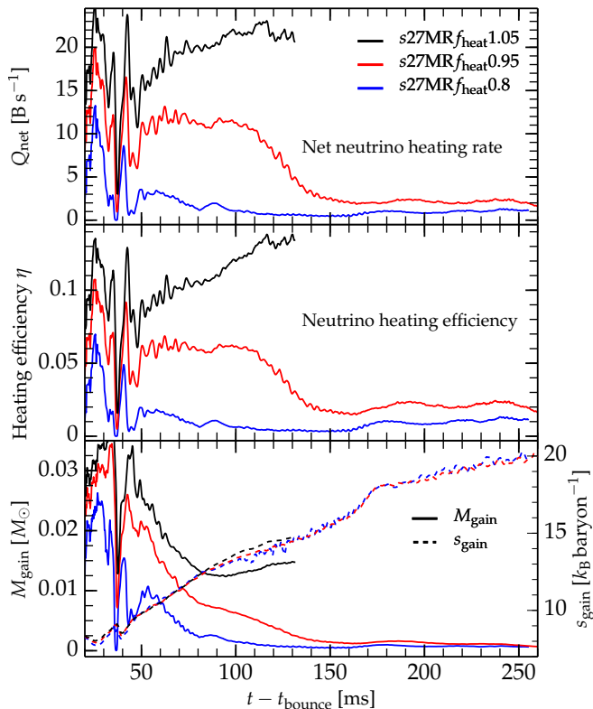
Figure 2. Integral quantities characterizing the strength of neutrino heating in models s27MR_{f_{\text{heat}}1.05} , s27MR_{f_{\text{heat}}0.95} , and s27MR_{f_{\text{heat}}0.8} with three different f_{\text{heat}} . Top panel: net neutrino heating rate Q_{\text{net}} (heating minus cooling) in \text{B s}^{-1} , where 1 Bethe = 10^{51} erg. Center panel: heating efficiency \eta defined as Q_{\text{net}} divided by the sum of the \nu_e and \bar{\nu}_e luminosities emerging from below the inner boundary of the gain region. Bottom panel: Mass M_{\text{gain}} (left ordinate) and average specific entropy s_{\text{gain}} (right ordinate) in the gain region. Q_{\text{net}} , \eta , M_{\text{gain}} all increase with increasing local heating factor f_{\text{heat}} .
