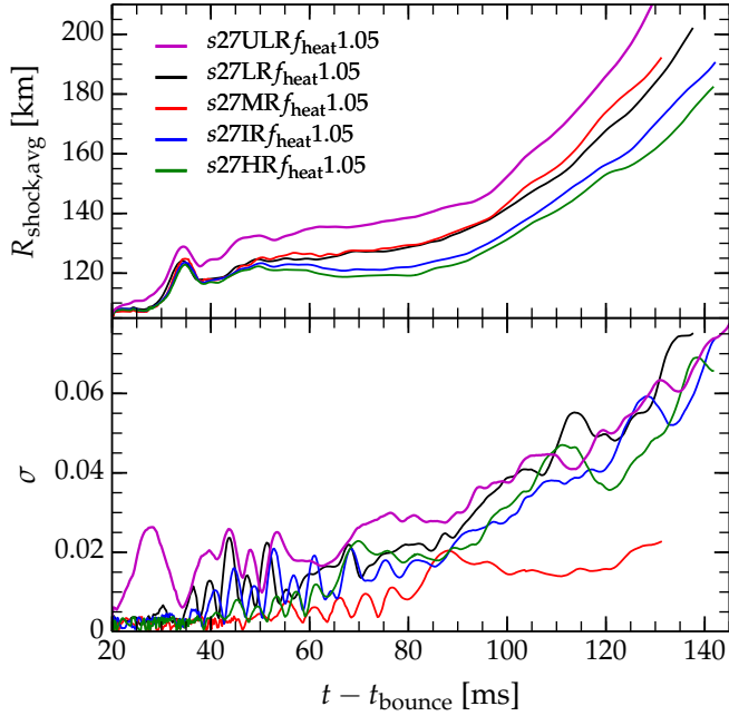
Figure 9. Top panel: Evolution of the average shock radii for five different resolutions in the strong neutrino heating regime ( f_{\text{heat}} = 1.05 ; see Table 1 for simulation details). Lower resolution leads to larger shock radii. Bottom panel: Evolution of the normalized root mean square deviation \sigma_{\text{shock}} of the shock radius from its angle averaged value for the same five models.
