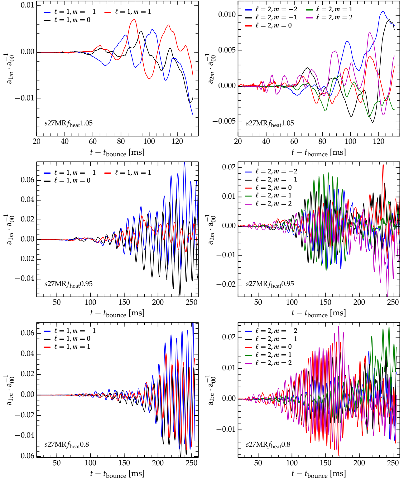
Figure 5. Normalized mode amplitudes a_{\ell m} \cdot a_{00}^{-1} of the shock front as a function of time for \ell = 1 (left panels) and \ell = 2 modes (right panels). We show amplitudes for models s27MR_{f_{\text{heat}}1.05} (strong neutrino heating, top row), s27MR_{f_{\text{heat}}0.95} (moderate neutrino heating, center row), and s27MR_{f_{\text{heat}}0.8} (weak neutrino heating, bottom row). Note that the range in postbounce time shown in the top row for the exploding model s27MR_{f_{\text{heat}}1.05} is different from the postbounce time covered for the two non-exploding models that develop strong long-lasting SASI oscillations.
