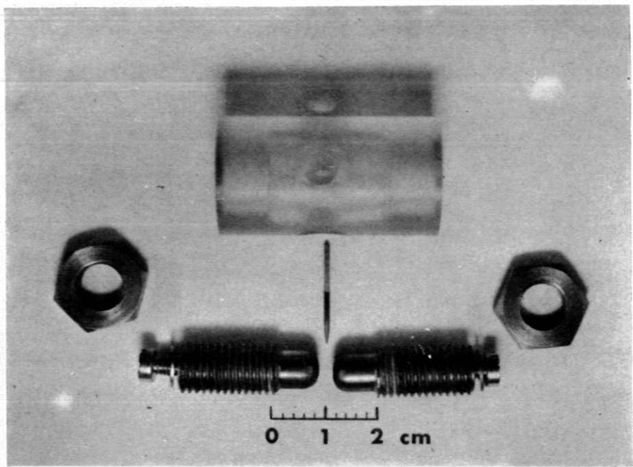
Fig.4 POINT-PLANE SPHERE-PLANE GAP
