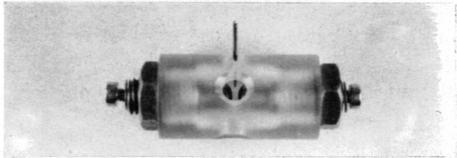
FIG.6 SPHERE-SPHERE GAP with CORONA ELEKTRODE
