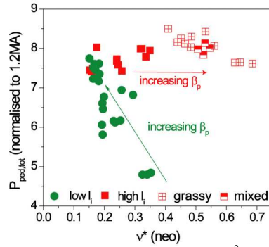
Figure 6: P_{ped} (normalised to I_p^2 ) for the high l_i and low l_i H-modes \beta_p scans.
