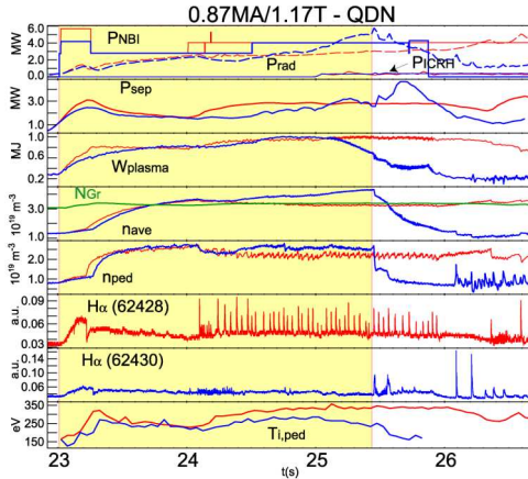
Figure 1: selected time traces for 2 pulses of the JET/Asdex-Upgrade identity experiments: in red pulse 62428 (Type I ELMs) and in blue, pulse 62430. The yellow box highlights the H-mode phase of #62430 until the loss of confinement due to core radiative collapse.
