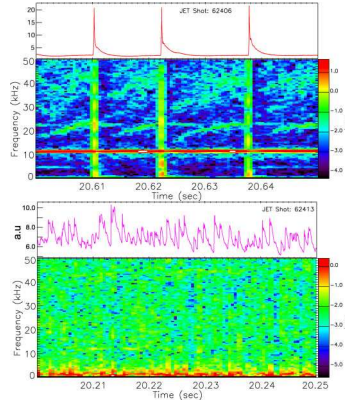
Figure 4: MHD spectrogrammes for #62406 (Type I ELMs, \beta_p \sim 1.35 ) and #62413 (Grassy ELMs, \beta_p \sim 1.9 )
