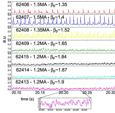
Figure 3: Divertor H_\alpha traces for the \beta_p scan in high l_i H-modes: Grassy ELMs observed for \beta_p > 1.6-1.7
