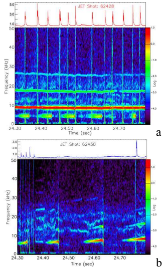
Figure 2: a): H_\alpha time trace and MHD spectrogramme showing Type I ELMs and core MHD, pulse #62428. b): #62430, same signals, showing the wb modes (broadband fluctuations, 10-25 kHz) and core MHD replacing the MHD activity typical of Type I ELMs.
