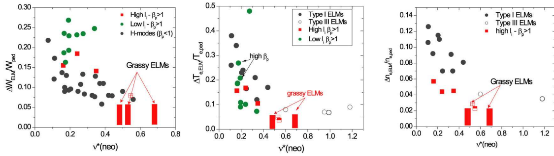
Figure 9: from left to right: ELM energy losses, normalised to W_{ped} , ELM temperature drop, normalised to T_{ped} and ELM density drop and, left, normalised to n_{ped} . Standard H-modes [3] in black, low- I_i H-modes in green, high- I_i H-modes in red. The red bars are calculated from estimated \Delta W_{ELM} , \Delta T_{ELM} and \Delta n_{ELM} , with the top of the bar being the upper value for those quantities.
