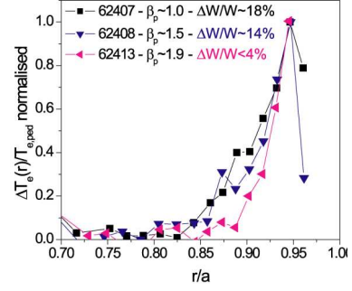
Figure 8: ELM perturbation of T_e profiles for low-medium and high \beta_p , high l_i H-modes.
