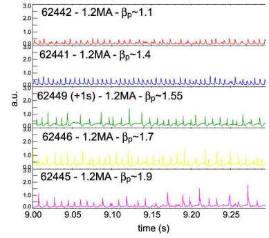
Figure 5: Divertor H_\alpha traces for the \beta_p scan in high l_i H-modes: Type I ELMs observed up to the highest \beta_p
