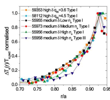
Figure 7: ELM perturbation of T_e profiles for standard H-modes: density scan (Type I and Type III ELMs)
