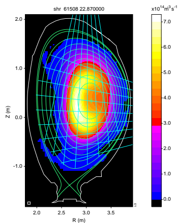
Figure 9. DT neutron profile for off-axis NBI into plasmas with n=1 fishbones (#61508).
