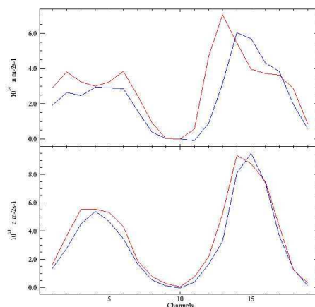
Figure 10. Measured vs TRANSP neutrons: top: #61508 with fishbones and off-axis T-blip ; bottom: off-axis T-blip case without fishbones/TAEs (#61344, B/I=3T/3MA)
