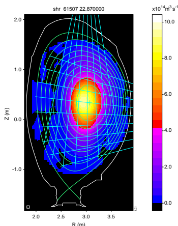
Figure 7. Tomographic reconstruction of DT neutron profile for on-axis NBI (#61507). Horizontal channels: 1(top) to 10(bottom), vertical ch.: 11 (inboard) to 19 (outboard)
