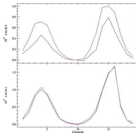
Figure 8. Comparison of measured (blue) vs TRANSP (red) profiles of DT neutrons 10 msec before end of T-blip: top: #61507 with fishbones and on-axis T-blip ; bottom: an example of on-axis T-blip case without fishbones/TAEs (#61341, B/I=3T/3MA)
