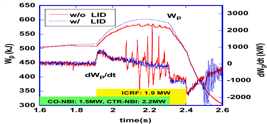
Fig.5 Time evolution of the stored energy and its time-derivative for two discharges without and with externally applied m=1/n=1 resonant helical field perturbations.
