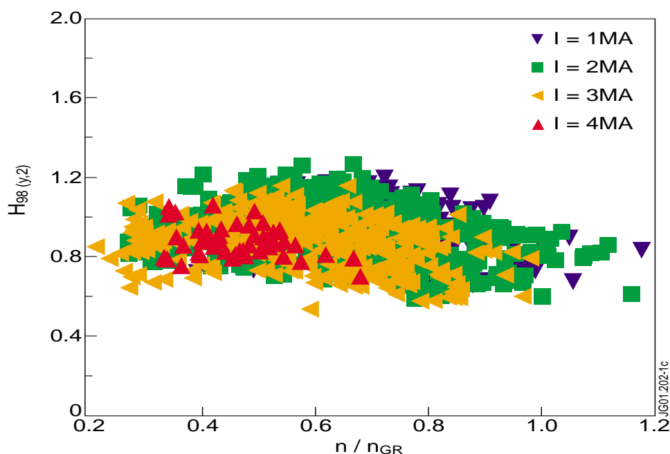
Fig. 1. H_{98} (\equiv \tau_{IH}/\tau_{E98}) versus n/n_{GR} , the data are grouped by current I in MA 0.5 < I < 1.5 , 1.5 < I < 2.5 , 2.5 < I < 3.5 and I > 3.5 .
