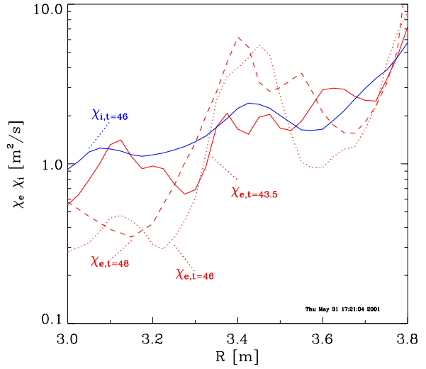
Figure 4: Electron and ion thermal diffusion ( \chi_e in red, \chi_i in blue) profiles from TRANSP. The eITB, seen as a local minimum in \chi_e , moves inward and intensifies. There is no sign of an ion ITB.
