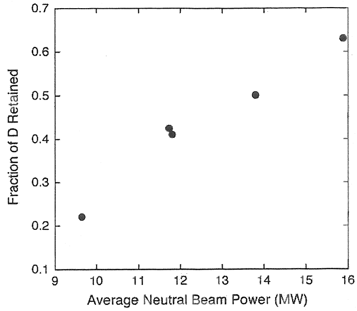
Figure 60. Fraction of deuterium retained in TFTR versus average neutral beam power.
