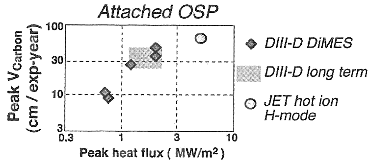
Figure 39. Net carbon erosion rate at the divertor strike-point vs. strike-point heat flux on JET and DIII-D. JET data [110] and DiMES at 1.5 \text{ MW}\cdot\text{m}^{-2} [521] were obtained with colorimetry. All other DiMES data come from depth-marked insertable probes [480, 530]. The DIII-D long-term results are from net changes in divertor tile height after 9 months of operation [491]. (OSP in the figure means outer-strike-point.); (reproduced with permission from [530].)
