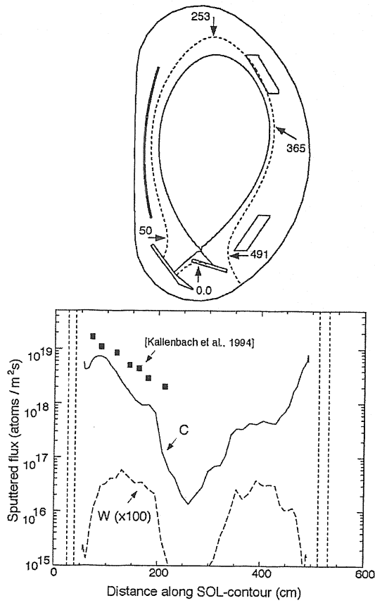
Figure 47. Distribution of the sputtered atom flux from the ASDEX-Upgrade vessel wall for carbon and tungsten wall material due to charge-exchange neutral sputtering as calculated from B2/EIRENE code calculations [156]. The carbon values can be compared to spectroscopically measured fluxes from the inner heat shield shown as solid squares [334]. The conditions in the divertor during erosion are: experiment: \langle n_e \rangle = 3 \cdot 10^{19} \cdot \text{m}^{-3} , calculations: n_e^{sep} = 5.2 \cdot 10^{19} \cdot \text{m}^{-3} .
