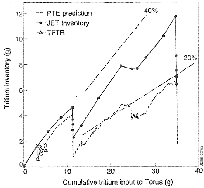
Figure 70. Tritium inventory in the torus versus cumulative tritium input during the JET DTE1 campaign; (reproduced with permission from [203].)
