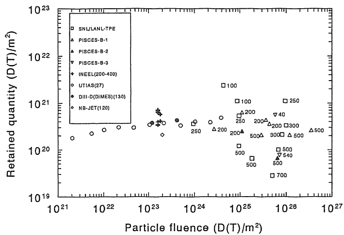
Figure 31. Retention of deuterium and tritium in Be as a function of incident particle fluence [427]. For purposes of comparing results from different experiments using different ion energies, the data have been scaled to correspond to an equivalent 100-eV deuterium ion energy. Numerical values next to the symbols and in the legend are specimen exposure temperatures, in degrees Celsius; (reproduced with permission from [427].)
