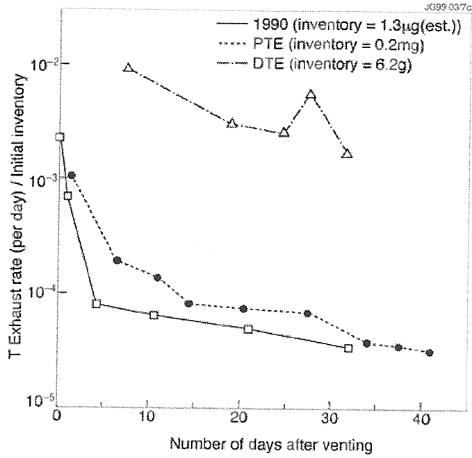
Figure 71. Rate of tritium release during air exposure of the torus at ambient temperature following the JET DTE1 campaign; (reproduced with permission from [203].)
