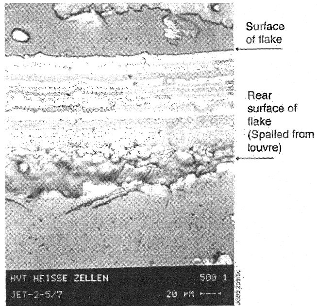
Figure 82. Polished cross-section of a flake from the JET Mk-IIA divertor, showing the layer structure. The scale marker on the figure is 20 \mu\text{m} , which makes the film thickness \approx 100 \mu\text{m} ; (reproduced with permission from JET.)
