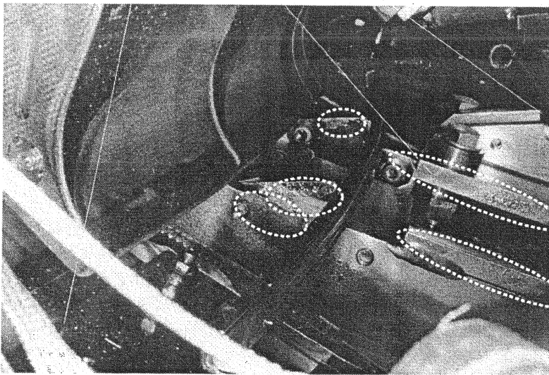
Figure 83. Location of flakes and films of carbon in ASDEX-Upgrade. The flakes were found below the divertor, whereas carbon films were found on the divertor structure. They are located at surfaces perpendicular to the magnetic field. The direction on the inner and outer divertor are reversed; (figure provided by V. Rohde - ASDEX-Upgrade, Garching.)
