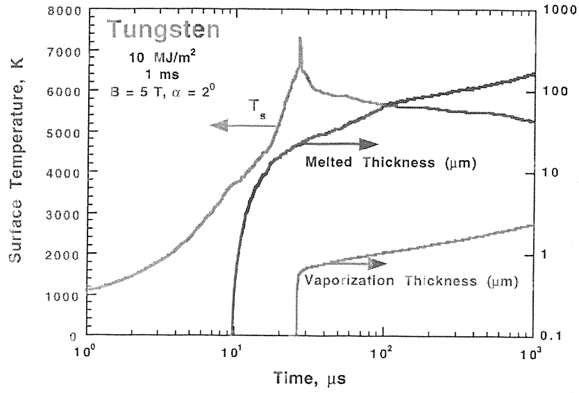
Figure 24. Time evolution of tungsten surface temperature, melt layer, and eroded thickness following a plasma disruption [363].
