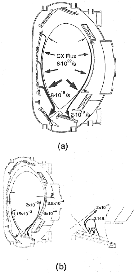
Figure 48. (a) Schematic erosion/re-deposition pattern of carbon wall material in the ASDEX-Upgrade divertor tokamak. For a total charge-exchange neutral flux of 8 \times 10^{22} D/s, the calculated C-impurity flux is of 8 \times 10^{19} C/s at the inner divertor and 2 \times 10^{19} C/s at the outer divertor. (b) Schematic of the erosion/re-deposition pattern of divertor material in a divertor tokamak as obtained from the ASDEX-Upgrade W divertor experiment; (reproduced with permission from [585].)
