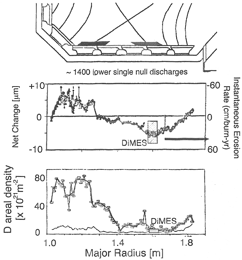
Figure 62. Retained deuterium and net erosion on tiles from the DIII-D divertor; (reproduced with permission from [721].)
