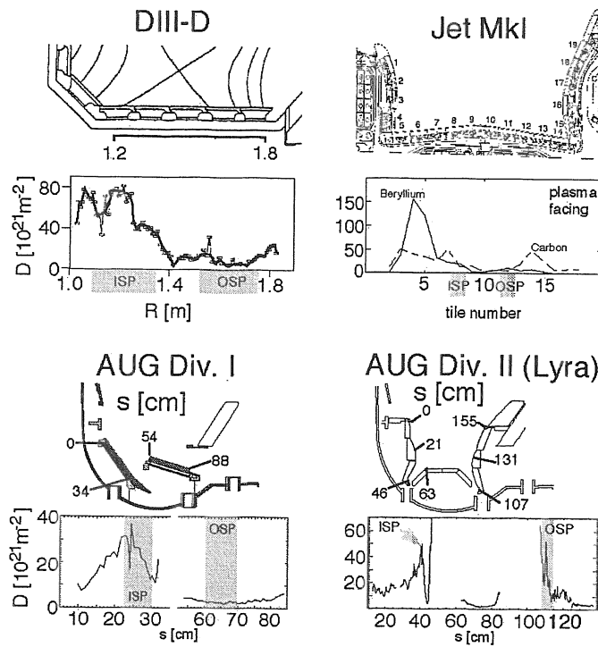
Figure 45. Re-deposition pattern of carbon onto the divertor plates of DIII-D, JET Mk-I, ASDEX-Uprade Div. I and Div. II LYRA, as documented by the D co-deposition pattern [63]. The inserts show the different divertor geometries.
