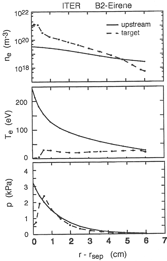
Figure 85. Results from a B2/EIRENE simulation of the ITER edge plasma [829]. r-r_{sep} is the distance from the last closed flux surface (outside mid-plane equivalent); (figure provided by A. Kukushkin, ITER.)
