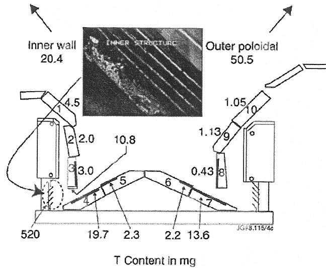
Figure 72. Distribution of tritium in the JET vessel in the shutdown following DTE1. The amounts at each location are integrated around the torus; (reproduced with permission from [758].). The photograph in the inset shows a typical region of the flaking deposition on the louvres at the inner corner of the JET Mk-IIA divertor; (reproduced with permission from JET.)
