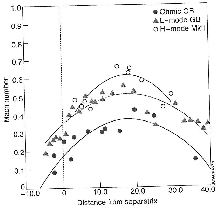
Figure 86. Flow in the JET SOL measured for different types of plasma. Using a Mach Probe on the Reciprocating Probe inserted near the top of the torus; (reproduced with permission from [841].)
