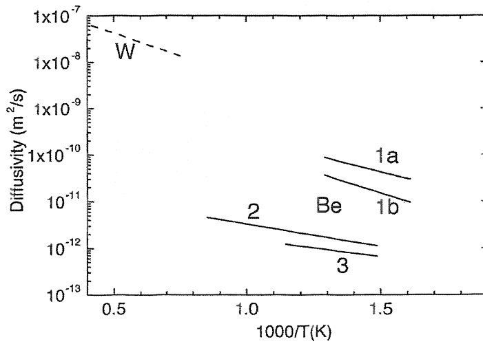
Figure 29. Measured diffusivity of hydrogen in tungsten (dashed line [403]) and beryllium (solid lines 1a&b [432], 2 [430] and 3 [433].)
