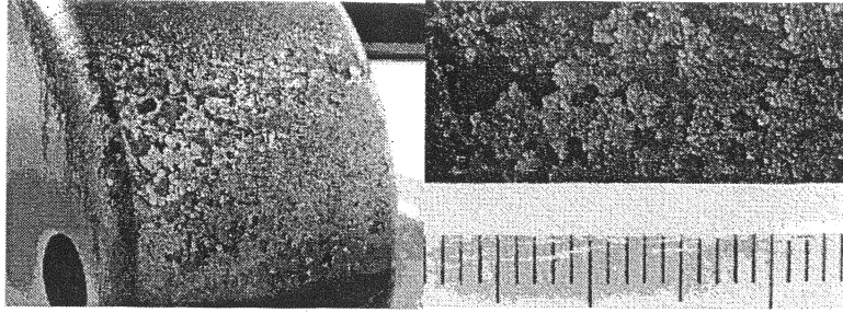
Figure 79. Photograph of the heavy deposition at the side of a TEXTOR limiter. The scale is in mm (visible are 23 mm) and refers to the detail of the flaking region shown on the upper right part of the figure; (reproduced with permission from TEXTOR.)
