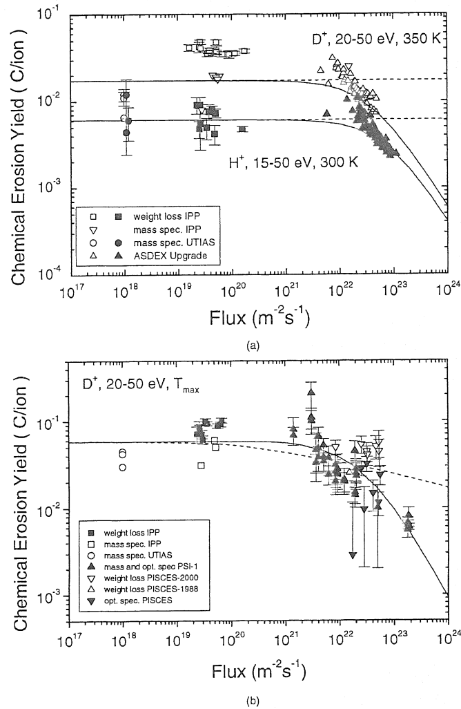
Figure 16. Flux dependence of the chemical erosion yield of carbon with deuterium ions near (a) room temperature and (b) T_{max} . The data combine weight loss and spectroscopic measurements from ion-beam experiments [288, 289, 302, 303], spectroscopic measurements from plasma simulators [295, 296, 304, 305] and from the ASDEX-Upgrade divertor [298]. The curves are fits to the data using the models described in [285, 293].
