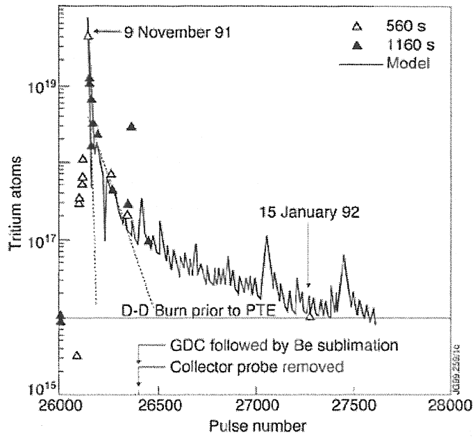
Figure 65. The number of tritium gas atoms released from the JET vacuum vessel as a function of pulse number for the PTE campaign and subsequent clean-up. The data are integrated for the first 560 s (open triangles) or 1160 s (closed triangles), and the solid curve is the prediction of a model; (reproduced with permission from [739].)
