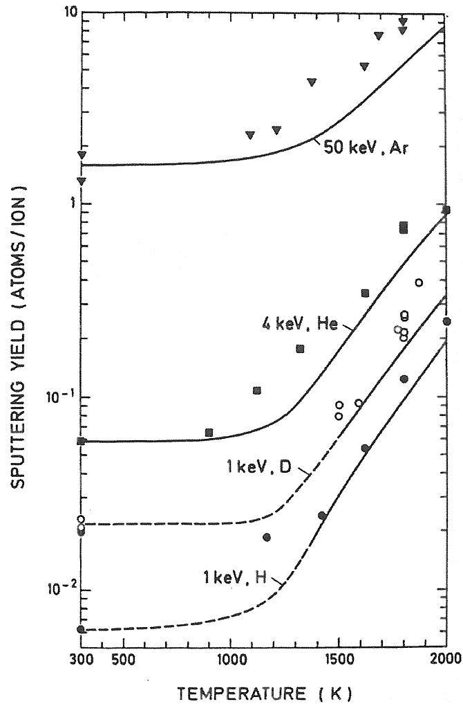
Figure 17. Temperature dependence of the sputtering yield of pyrolytic graphite by H^+ , D^+ , He^+ , and Ar^+ in the temperature range of RES. Solid curves are from the model described in Ref. [330]; (reproduced with permission from [330].)
