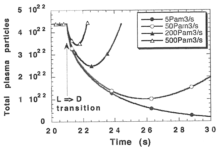
Figure 91. Density behaviour of deuterium during a typical limiter to divertor transition in the 1998 ITER design for various values of the fuelling rate; (figure provided by M. Sugihara, ITER.)
