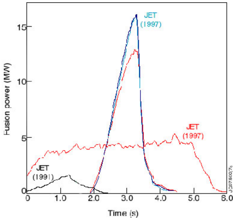
Figure V: Fusion energy production in the Joint European Torus (JET)[11].
