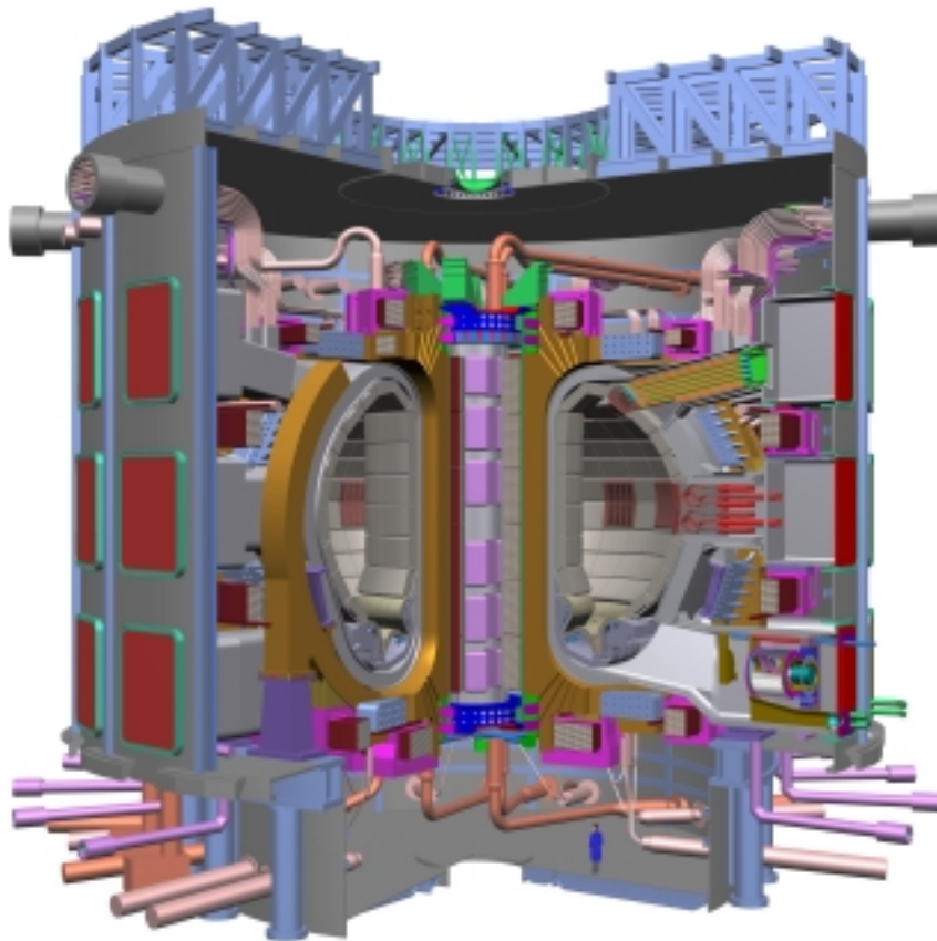
Figure VII: Sketch of the ITER-FEAT Experiment (photo ITER)
