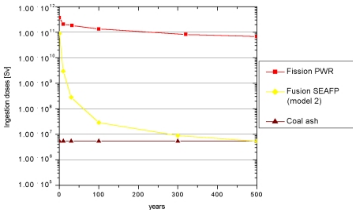
Figure X: Development of radiotoxicity for a fusion plant, a fission plant and the ash of a coal plant. It is assumed that all the plants produce the same quantity of electricity. The volume of coal ash is of course 2-3 orders of magnitude greater than that of fusion or fission waste.
