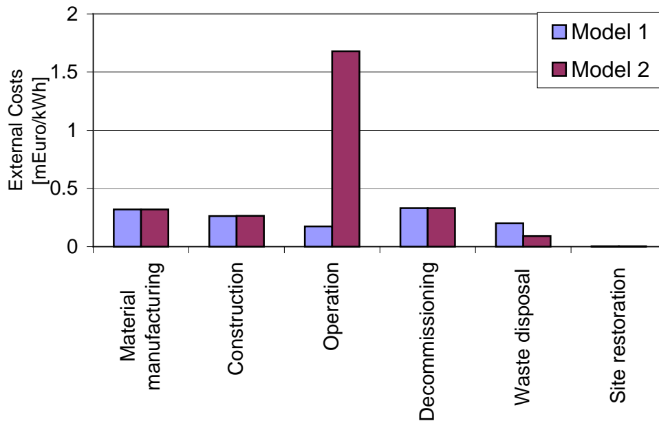
Figure XI: External costs of fusion [41].
