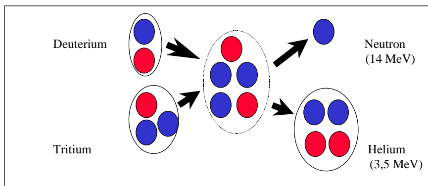
Figure I: Schematic of the fusion reaction in which deuterium and tritium form a helium atom and a neutron. Mass is lost in the reaction and energy gained.
