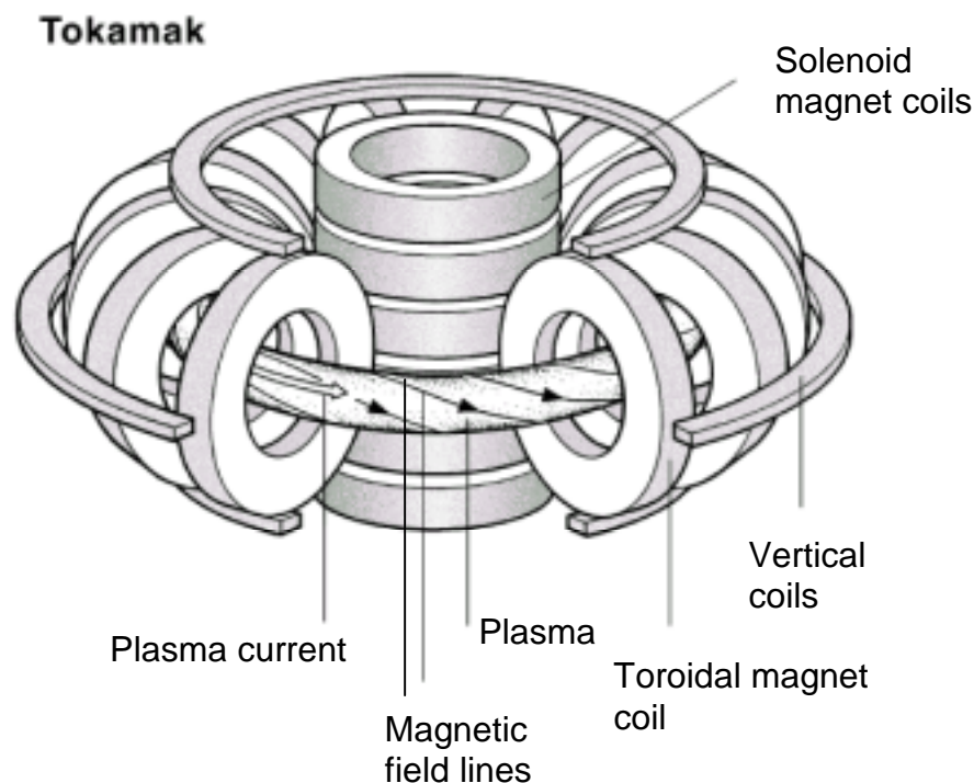
Figure II: The tokamak has so far been the most successful magnetic confinement scheme. The magnetic field cage - necessary to confine the charged particles - is produced by the superposition of a toroidal magnetic field and a poloidal magnetic field produced by a current in the plasma.
