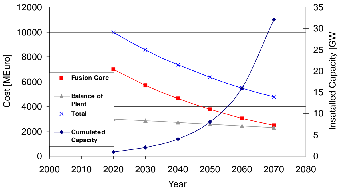
Figure IX: Learning curves for fusion power plants [29].
