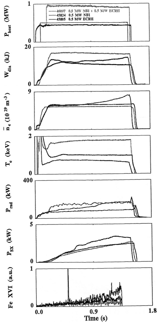
Figure 6: Overview of discharge evolution for a central electron density of 6 \times 10^{19} \text{ m}^{-3} with 0.5 MW NBI, 0.5 MW ECRH and combined heating of 0.5 MW NBI and 0.5 MW ECRH. Density control is possible with combined heating in comparison to the NBI discharge.
