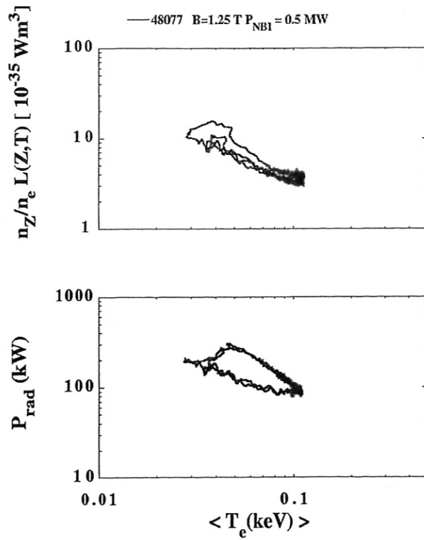
Figure 13: Total radiated power and the normalized radiated power of Eqn. 21 for the P_{NBI} = 0.5 MW discharge at B = 1.25 T plotted as a function of derived mean temperature. The observed hysteresis in radiated power is therefore due to the density collapse at the density limit.
