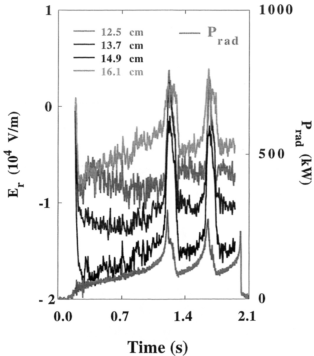
Figure 3: Time evolution of radial electric field measurements at various radii showing that the rise in radiated power and the concurrent plasma cooling is accompanied by a reduction in the magnitude of the radial electric field.
