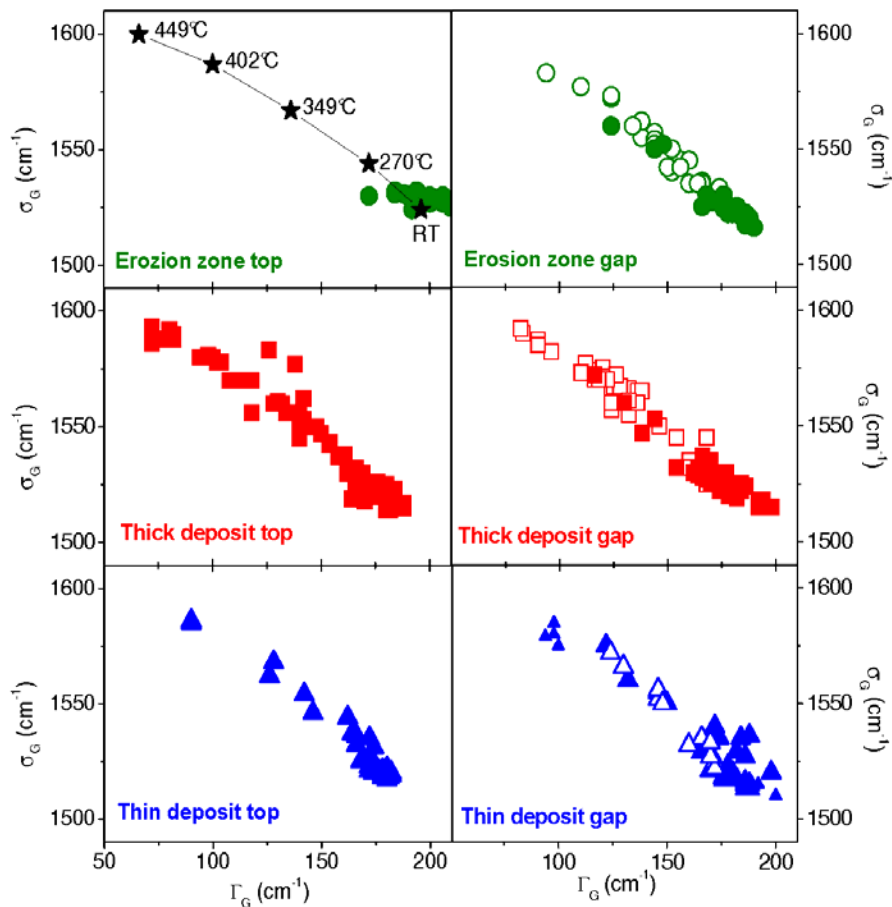
Figure 2. \sigma_G against \Gamma_G plot for tiles coming from the three zones (left side: top surfaces, right side: gap surfaces), compared to a heat treated a-C:H layer. Empty symbols correspond to spectra recorded on the gap surface close to the top surface (for details see text).
