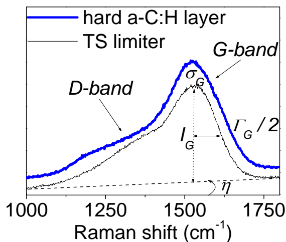
Figure 1. Raman spectrum obtained for a plasma-deposited hard amorphous carbon layer compared with a spectrum recorded on the top surface of a tile from the thick deposit region. \sigma_G , \Gamma_G , I_G are the G band wavenumber, full width at half maximum and intensity, respectively, and \eta is the slope of the photoluminescence background.
