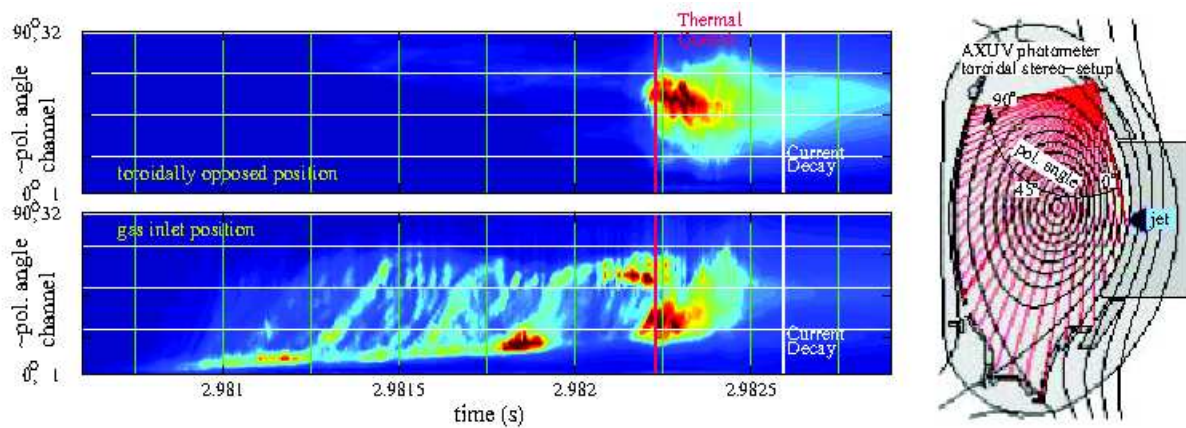
Figure 11. Temporal and spatial development during a neon-MGI mitigated disruption in a toroidal position opposite to the MGI valve and in sector of the MGI valve for # 24442 [43]. The right figure shows the geometry of the viewing lines, from this, a poloidal motion of filaments over the plasma top towards the high field side can be inferred in the gas valve sector.
