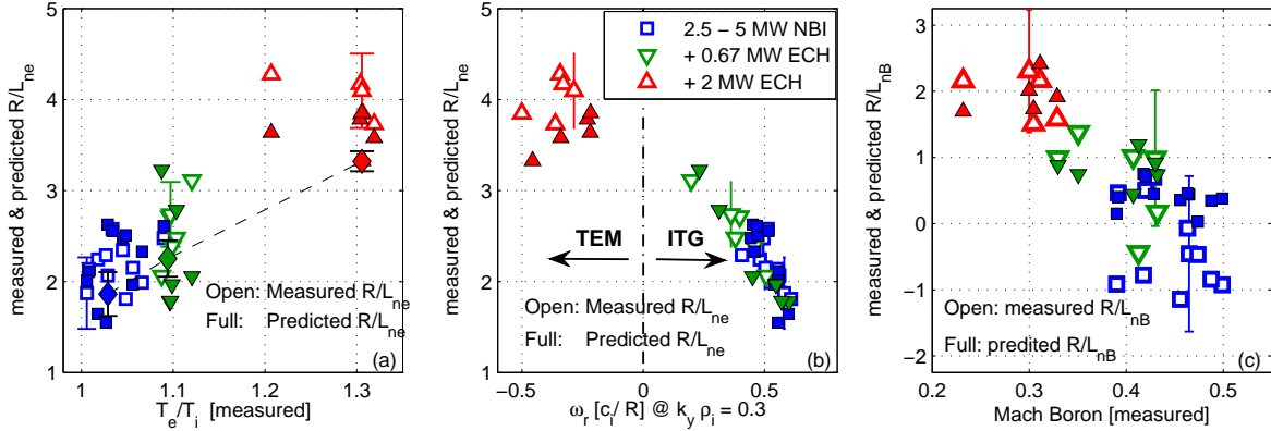
Figure 6. Analysis of representative cases of the three heating phases corresponding to figure 5 at half radius. a) Comparison of predicted quasi-linear GS2 (full symbols with squares, triangles pointing down and up), nonlinear GYRO (diamonds connected by a dashed line) and measured (open symbols) values of R/L_{ne} as a function of the temperature ratio T_e/T_i . b) Predicted and measured R/L_{ne} versus the real frequency of the most unstable mode at k_y \rho_i = 0.3 . c) Normalized inverse gradient length R/L_{nB} of B^{5+} ions versus the toroidal Mach number [19]. This figure has corrected an error in the theoretical calculations shown in corresponding IAEA viewgraph Fig. 6 in [23]. The correct mode rotation in the high ECRH power phase is negative, indicating dominant TEM instabilities.
