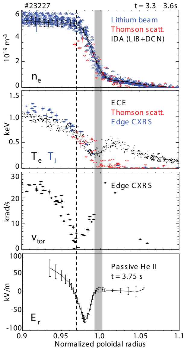
Figure 1. Pedestal profiles of the electron density (the solid line shows the result of integrated data analysis (IDA) of Lithium beam and DCN interferometer data), electron and ion temperature, toroidal angular rotation frequency and radial electric field for the inter-ELM phase of a type-I ELMy H-mode.
