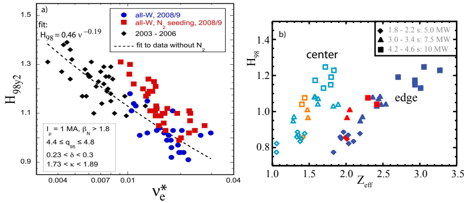
Figure 7. a) H_{98(y,2)} confinement factor vs. collisionality for different H-mode discharges with and without nitrogen seeding. b) H-factor H_{98(y,2)} for discharges with/without (blue/red) nitrogen seeding versus Z_{eff} at \rho_{pol} = 0.2/0.9 (open/full symbols) [25].
