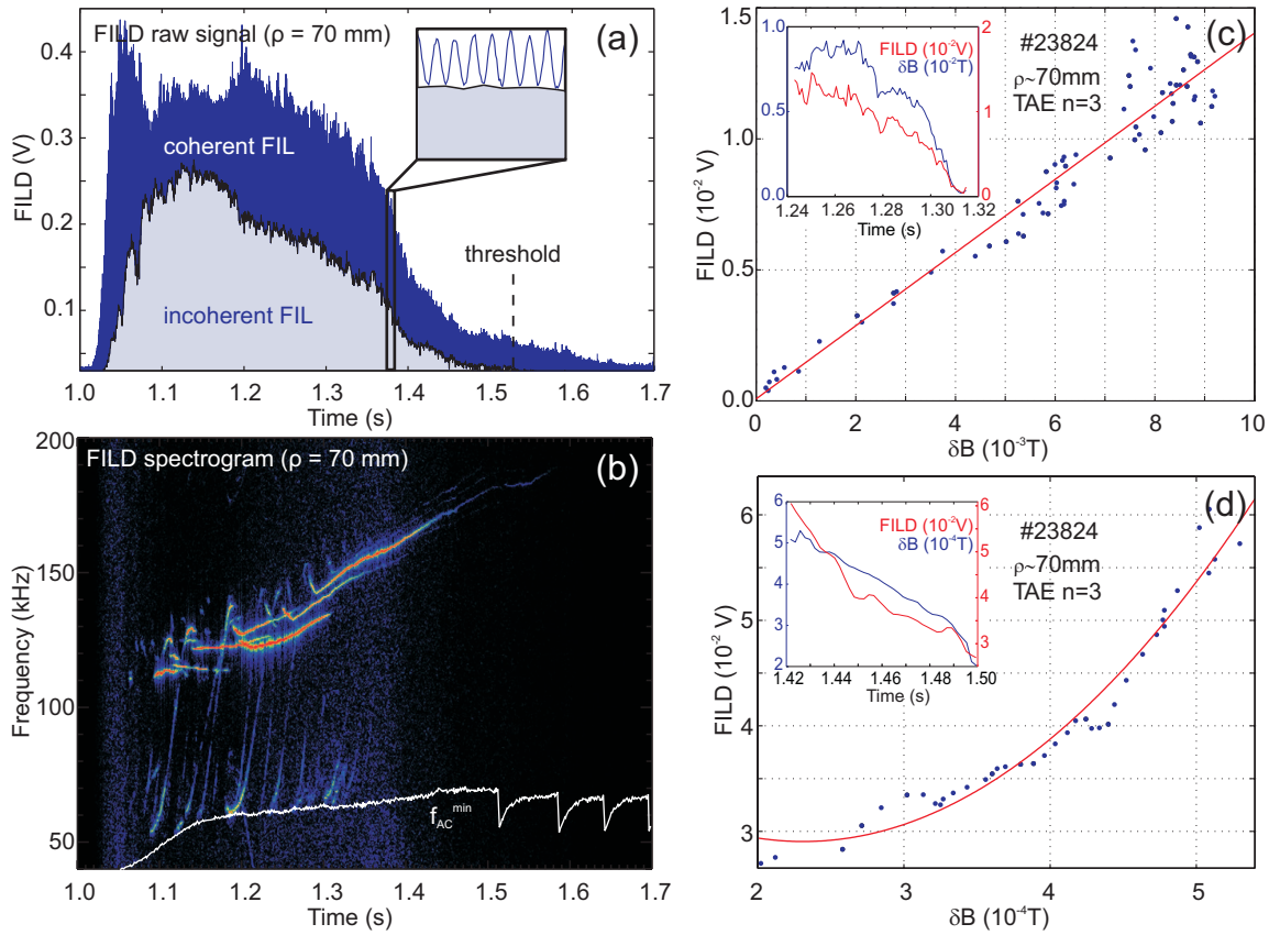
Figure 8. a) Raw signal of the fast ion loss detector during a pulse with strong MHD activity. b) Spectrogram showing AC and TAE activity. The geodesic frequency f_{AC}^{min} [27] is indicated in white for reference. c) Linear dependence of coherent FIL signal on magnetic fluctuating amplitude \delta B interpreted as convective losses. d) Non-linear (offset-quadratic) dependence of incoherent FIL signal on \delta B interpreted as conductive losses.
