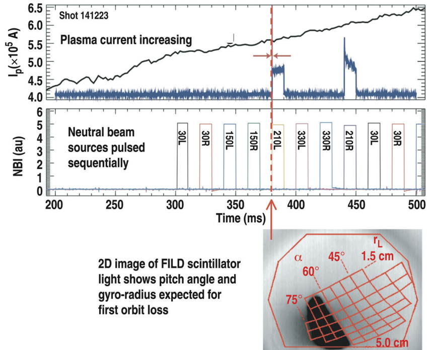
Fig. 2. First orbit losses were observed during pulsed operation of neutral beam sources while slowly increasing plasma current.
