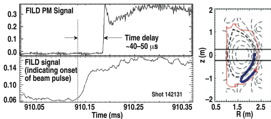
Fig. 3. The measured loss signal is delayed by \sim 40\text{--}50 \mu\text{s} , as expected based on the transit time for first orbit losses.
