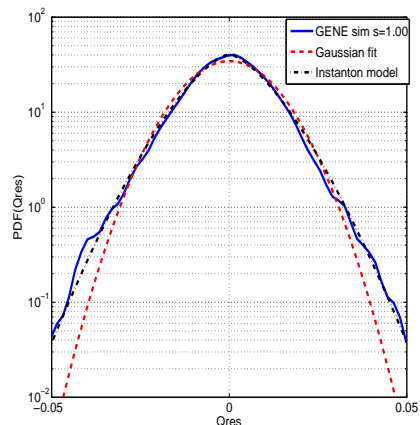
FIG. 4: Comparison of the numerically estimated PDF (blue line) against the analytically prediction (dashed dotted black line) and the best fit Gaussian (dashed red line) for \hat{s} = 1.0 .
