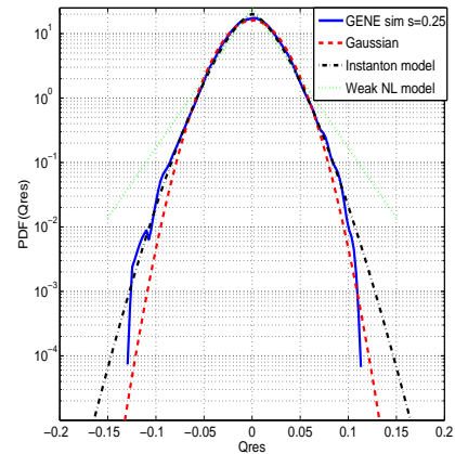
FIG. 3: Comparison of the numerically estimated PDF (blue line) against the analytically predicted instanton model (dashed-dotted black line) and weak non-linear model (dashed green line) compared to the best fit Gaussian (dashed red line) for \hat{s} = 0.25 .
