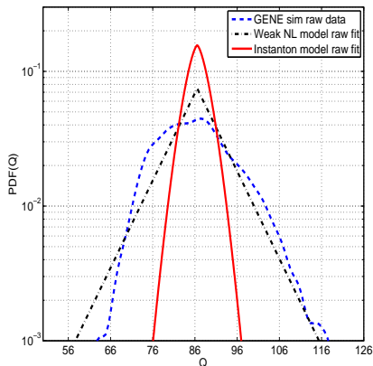
FIG. 2: The numerically estimated PDF of heat flux (dashed blue line) in comparison with the analytically predicted instanton method (red line) and the weak non-linear model (dashed-dotted black line) at magnetic shear \hat{s} = 0.25 .
