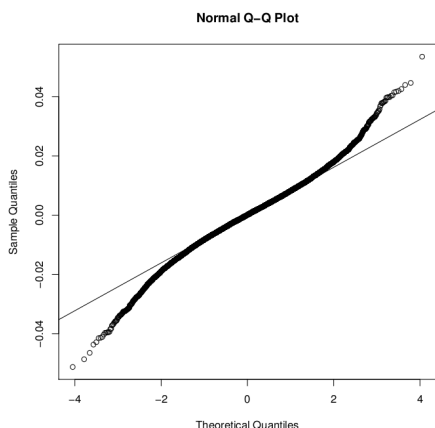
FIG. 1: Normal quantile-quantile plot showing strong deviation of the residual PDF from Gaussian statistics, in view of the enhanced tails representing about half of the sample.
