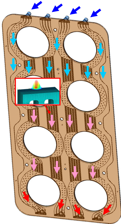
Fig.5 View of the source case Drivers Plate cooling channels
