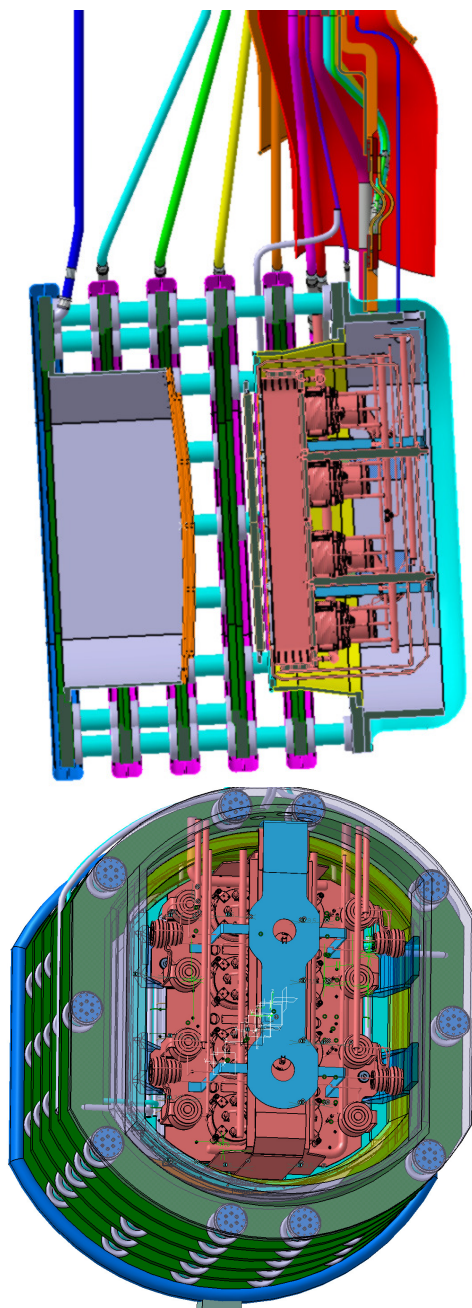
Fig.6 Integration in the beam source
