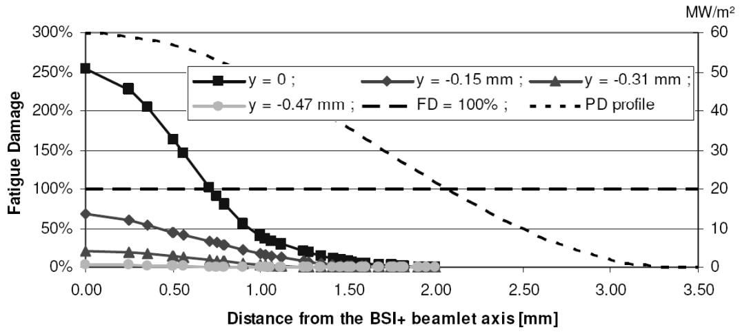
Fig.7 Fatigue life assessment for Drivers Plate most stressed areas
