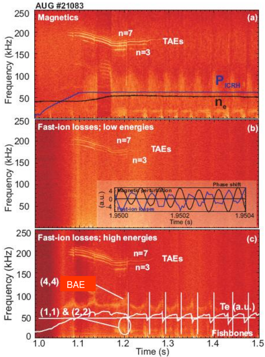
Fig. 6: Fast particle losses due to modes driven by energetic particles: magnetic perturbation spectra (a) and fast ion loss detector spectra (b) and (c) show the same frequencies. The phase relation between them is shown in the insert in (b) for a TAE. At high particle energies (part (c) of the diagram), also a Beta-induced Alfvén Eigenmode (BAE) is identified.
