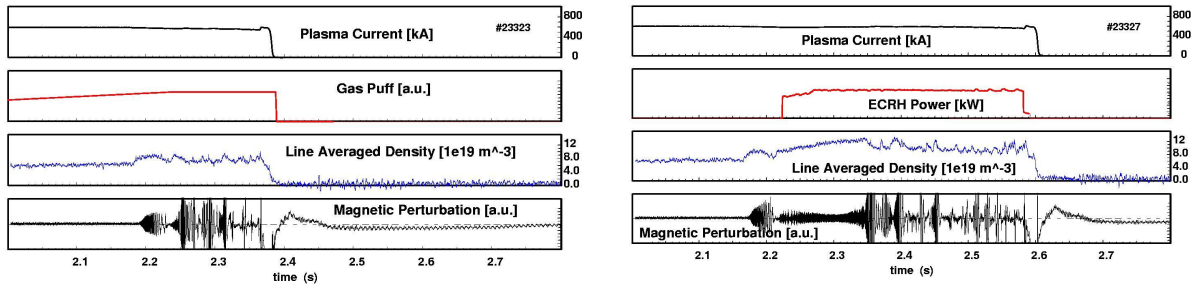
Fig. 5: Delay of a density limit disruption by injecting 0.6 MW ECRH at the q=2 surface (right panel). A transient phase with low MHD activity occurs in which the density can be substantially increased.
