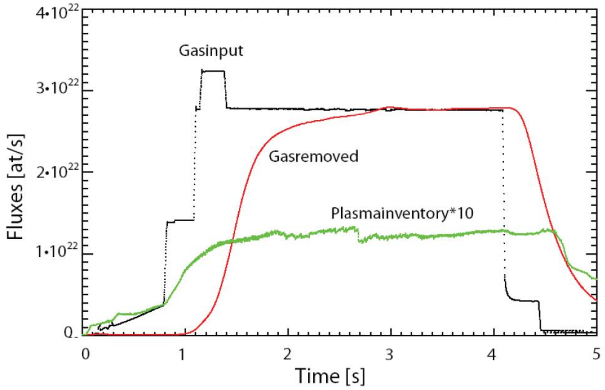
Fig. 2: Gas balance for a high density AUG discharge with W-wall. Wall saturation is achieved in the late flat-top phase (time interval 3-4 s).
