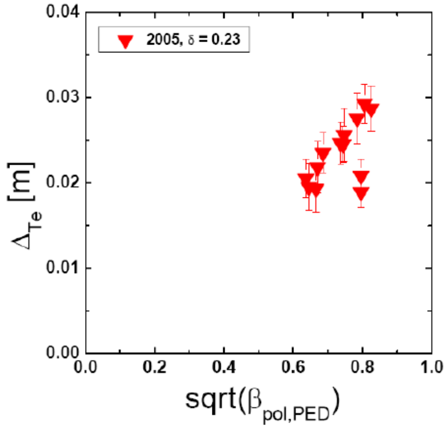
Fig. 3: The T_e pedestal width scales with \beta_{\text{pol, ped}}^{1/2} in improved H-mode at low \delta .
