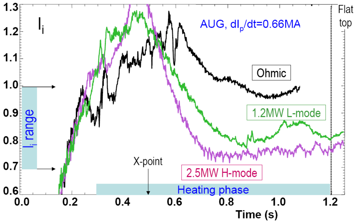
Fig. 9: Variation of the I_i value in flat top by using different heating schemes during ramp-up. The ITER target range is indicated in blue.
