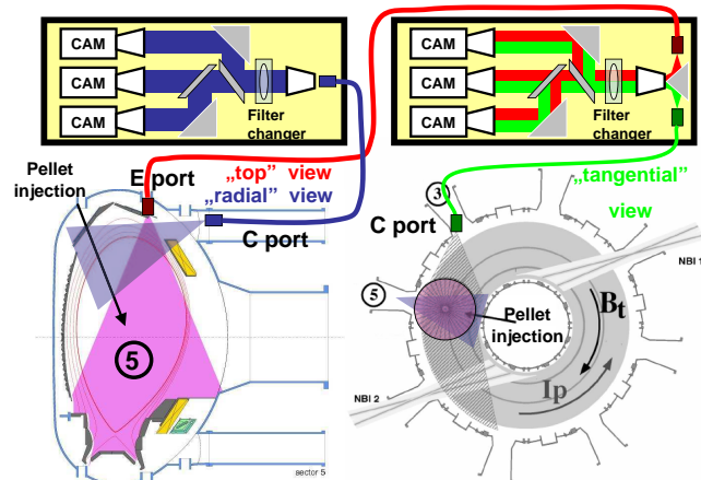
Figure 1: ASDEX Upgrade experimental set-up: cameras detect the pellet cloud radiation from radial ('radial view'), toroidal ('tangential view') and vertical ('top view') directions.
