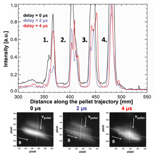
Figure 3: Line-cut - along the designated pellet trajectory - of multiple exposure images made with different delay times (upper part) and images with different delay time about the cloud No. 1.
