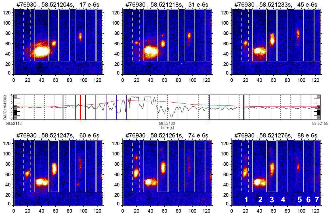
Figure 5: Mirnov coil signal (middle) during a pellet triggered ELM with its high frequency envelope (red) and the calculated ELM onset time (over-plotted red vertical line). The black vertical line denotes the ELM MHD onset. The six plots around are successive frames of the fast camera, their frame times are marked on the Mirnov coil signal by blue vertical lines. The white boxes are used for image processing encircling the left ILA limiter (1), the pellet ablation location (2), the right ILA limiter (3), inter limiter areas (4,6) and middle of the antenna (5) which acts as limiter and the edge of the last limiter seen on the images (7).
