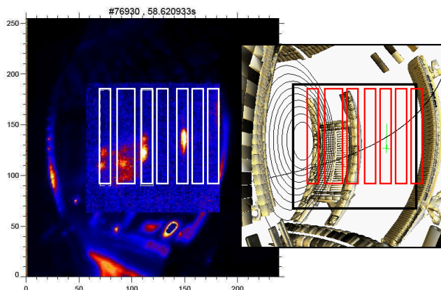
Figure 4: The view of the fast visible imaging on JET. Left a slow framing image showing the whole cross section is over-plotted with a fast framing one. On right the computer model of the view together with equilibrium magnetic surfaces of the poloidal plane of the pellet injection and a field line started where the pellet crossed the separatrix. The white (red on right) boxes are used during the image processing.
