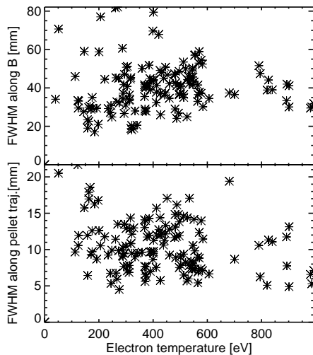
Figure 2: The FWHM of the clouds in the database along the magnetic field line crossing the cloud (upper part) and along the designated pellet trajectory (lower part).
