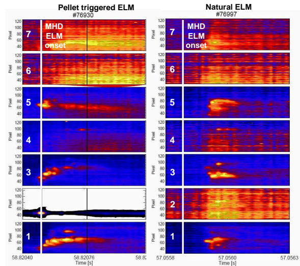
Figure 6: The time evolution of the distribution of box radiation for the above defined seven boxes for a triggered ELM (left) and for a natural ELM (right). The MHD ELM onset is also over-plotted (white vertical line).
