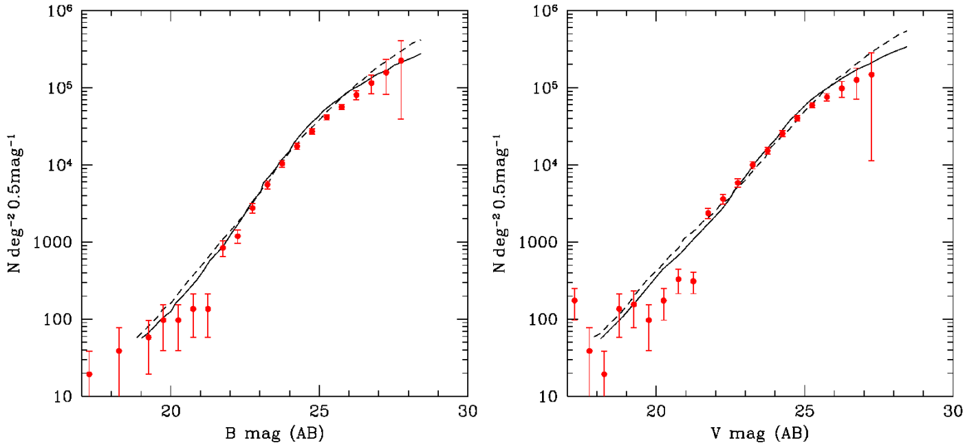
Fig. 14. Measured surface densities in the B and V band (red points), plotted with number counts from the simulations of Nagashima et al. (2005). The solid and dashed lines represent the strong and weak supernova feedback cases respectively. The faint end slope of the weak feedback model is in better agreement with the B-band data, while the the strong feedback model is in better agreement with the V-band data.
