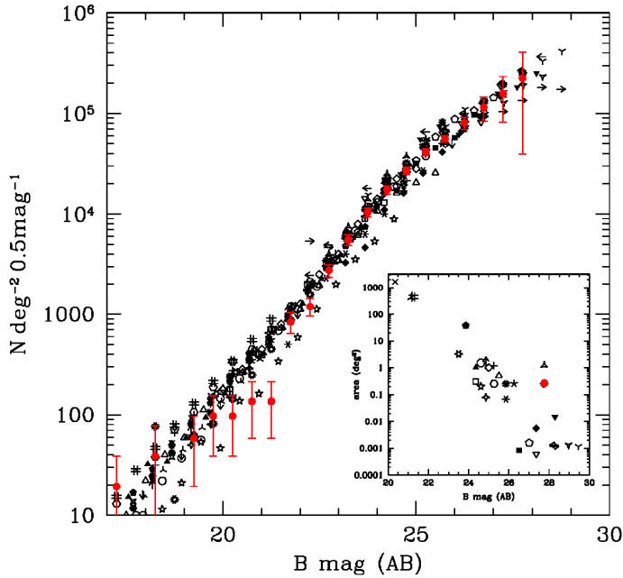
Fig. 10. Same as Fig. 9 but for the B-band
