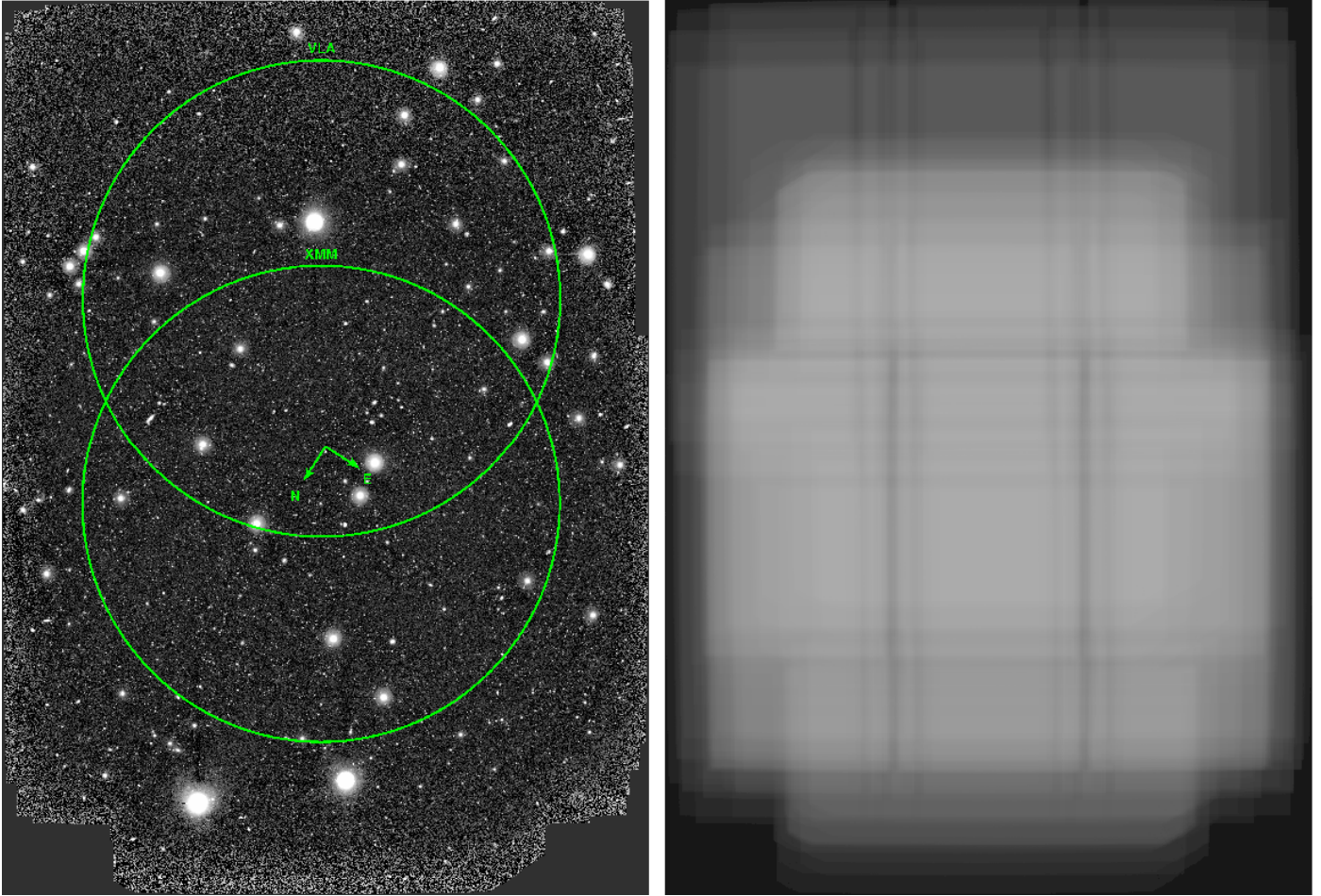
Fig. 4. Final U-band image and corresponding exposure map. The image covers both the XMM and the VLA fields, which are marked with 10' -radii circular regions, close to their typical widths. The highest exposure is in the overlapping region between them.
