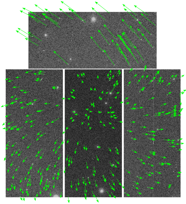
Fig. 2. Astrometrical solutions applied to an exposure image of 11 June 2007 (U-band). The image has been bias and flat calibrated but no astrometrical solution has been applied. The arrows represent the shifts to the calibration sources exaggerated 8 times. To compensate for the distortion we dealt with each chip separately and after applying an initial shift we fitted a 4th order polynomial to the corrections. The corrected images have an rms scatter of \sim 0.2 arcsec
