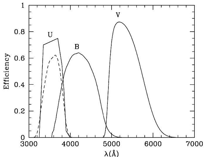
Fig. 1. Transmission curves of the filters used (U-spec - B-Bessel - V-Bessel) are shown by continuous lines. The dotted line represents the U-Bessel filter available on the LBC. We have chosen the U-spec filter for the U-band on grounds of its better efficiency and more uniform spectral coverage. These curves represent the filters’ responses without accounting for the detectors’ responses or the atmosphere. The detectors’ responses are slightly different for the two arms of the telescope which might have an effect in the V-band.
