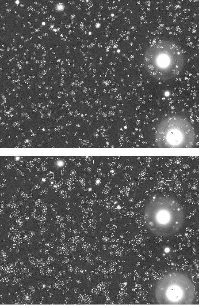
Fig. 5. Apertures of extracted sources in the U image. The upper panel shows the “dual mode” results and the lower the “single mode” (see text) Note that the detection efficiency near the bright object as, the deblending efficiency and the apertures of faint sources are much better in “dual mode”, but the apertures of bright objects are more reasonable in “single mode”.
