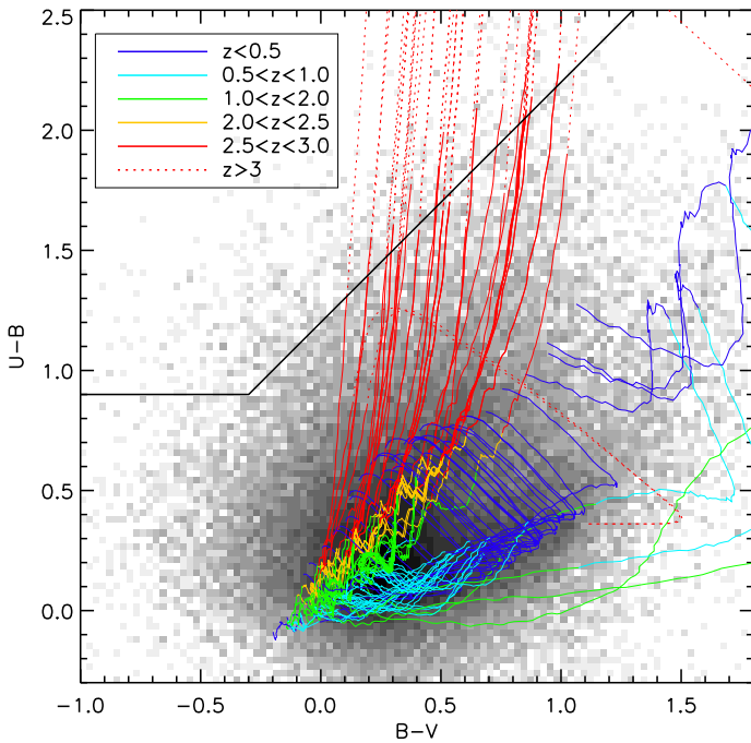
Fig. 12. The same plot as Fig. 7, but with SEDs created with the GISEL98 code (Bruzual & Charlot, 1993) with different metallicity and extinction properties (see Bolzonella et al., 2000). We use elliptical, irregular and spiral tracks, colour-coded with redshift ranges. The bulk of the distribution is reproduced with spiral and irregular tracks at redshift 0.5 < z < 2.5 . The z \gtrsim 3 region is also marked.
