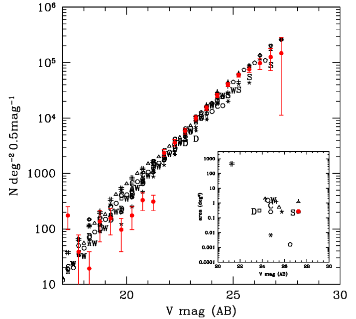
Fig. 11. Same as Fig. 9 but for the V-band
