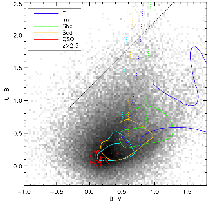
Fig. 7. Optical colours of the Lockman hole sources in the AB system. The greyscale represents the density of sources detected in all three bands are plotted. The black line marks the selection area of U-dropout sources with redshift z \geq 3 (see Fig. 12 and § 6.2). Dotted are the tracks above z = 2.5 , where the SEDs are not well sampled. The coloured lines represent tracks of different SED templates: blue line for ellipticals, cyan for irregular, green for Sbc, yellow for Scd, and red for QSO.
