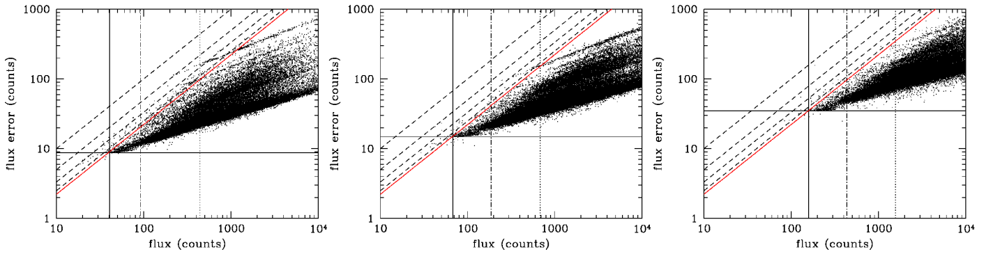
Fig. 6. Flux error versus flux diagrams for source detections in the U, B, and V filters. The zero-point magnitudes for the three filters are 32.911 \pm 0.013 , 33.830 \pm 0.014 , and 34.110 \pm 0.011 respectively. The dashed lines represent signal-to-noise ratios of 1, 2, and 3, and the red solid lines represent the (empirical) limit of the source extracting algorithm used ( 4.5 \sigma ). The horizontal and vertical solid lines mark the minimum flux and the respective minimum flux error of the faintest sources extracted. The dotted and dash-dotted lines mark the 50% efficiency limit and the limit of the number count analysis respectively.
