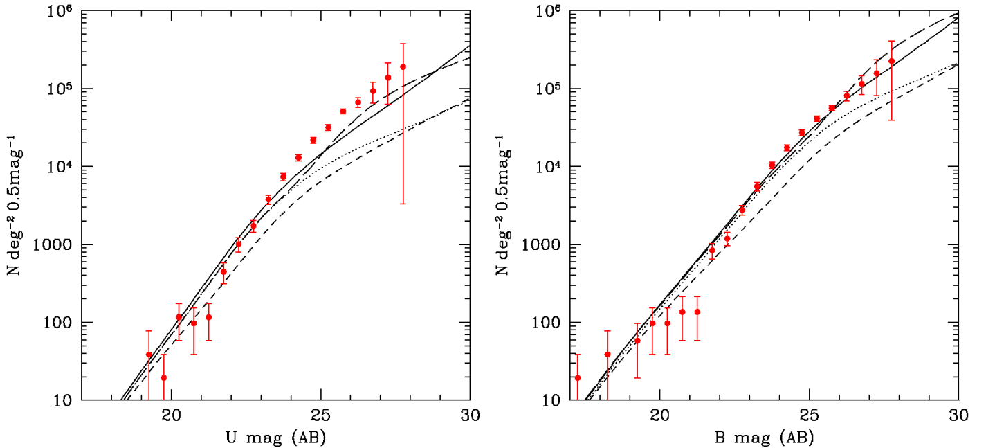
Fig. 13. Measured surface densities in the U and B band (red points), plotted with evolution models from Metcalfe et al. (1996) and Metcalfe et al. (2001). The short-dashed lines represent the pure luminosity evolution model, the long-dashed lines the same model with the inclusion of a population of star-forming dwarf galaxies, and the solid lines the same pure luminosity evolution model with a steep faint-end slope of the luminosity function. The latter is in very good agreement with the B-band counts, while the U-band counts are under-predicted by all models.
