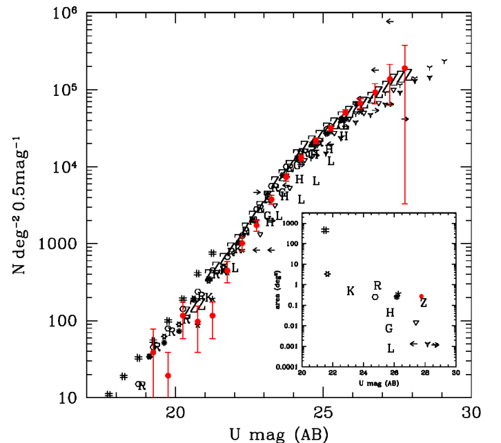
Fig. 9. U-band surface density distribution corrected for efficiency and spurious detections. The data points of this study (seen in Tab. 4) are plotted in red dots, while various symbols represent the results of other surveys found in the literature (see Tab. 3), corrected to AB magnitudes. The inner plot shows the depth of each survey (in terms of secure number count measurements) with respect to its width.
