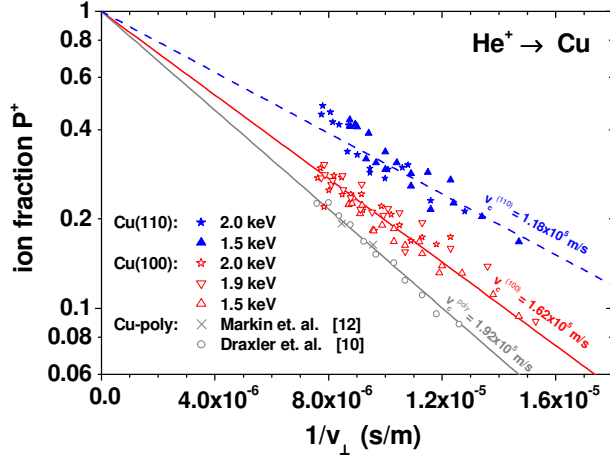
Fig. 2: Ion fraction P^+ of \text{He}^+ scattered from Cu(110) (full symbols), Cu(100) (open asterisks and triangles) and polycrystalline Cu (crosses and open circles) in the AN regime, as a function of 1/v_{\perp} = 1/v_{\perp, \text{in}} + 1/v_{\perp, \text{out}} . Also shown are single exponential fits (see Eq. (1)) with characteristic velocity values as indicated in the figure (for details see text).
