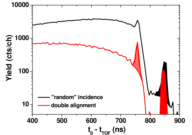
Fig. 1: Experimental spectra are shown as a function of the inverse time-of-flight t_0 - t_{TOF} , where t_0 is a constant and t_{TOF} the time-of-flight for 5 keV \text{He}^+ ions and a Cu(100) surface. The spectra refer to double alignment geometry ( \alpha = 0^\circ , \beta = 51^\circ , azimuth in (001) direction, grey line (red online)) and to “random” geometry ( \alpha = 25^\circ , \beta = 26^\circ , azimuth in (001) direction, black line). The surface peak intensities of ions and neutrals after subtraction of a linear background are indicated as hatched and filled areas, respectively.
