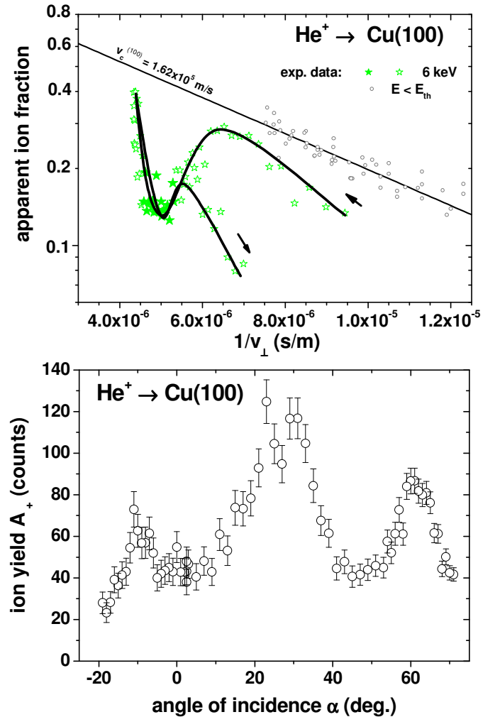
Fig. 3a: Apparent ion fraction P^+ of 6 keV \text{He}^+ scattered from Cu(100), as a function of 1/v_{\perp} = 1/v_{\perp, \text{in}} + 1/v_{\perp, \text{out}} . Full asterisks refer to double alignment geometry, open asterisks to scattering out of double alignment. The
