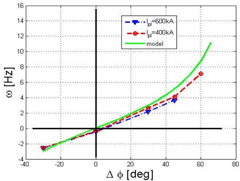
FIG. 4 (color online). Dependence of mode rotation on phase shift between the mode and the external perturbations. Full line (green online) represents the result of the model discussed in the text; circles and triangles represent the experimental rotation speeds obtained for two levels of plasma current.
