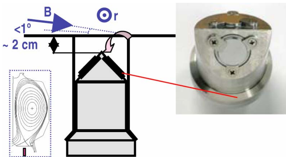
Fig. 2: Illustration and picture of DiMES mirror sample.
