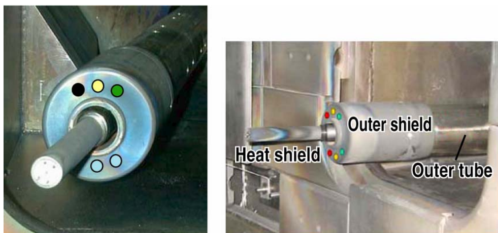
Fig. 4: MiMES location and possible installation of material samples on the graphite shield of the mid-plane fast probe.
