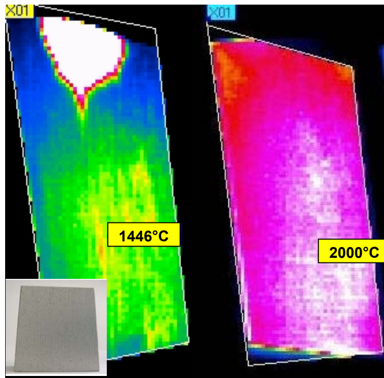
Fig. 3: W-coated tile (lower left corner) and infrared images during high heat flux testing: 10 \mu m coating, 10s pulse at 4 MW/m 2 (left) and 200 \mu m coating, 4s pulse at 11 MW/m 2 (right). The given temperatures correspond to the centre of the hydrogen beam. The bright white area in the tile on the left is caused by delaminating of the coating, which overheats beyond the dynamic range of the infrared camera.
