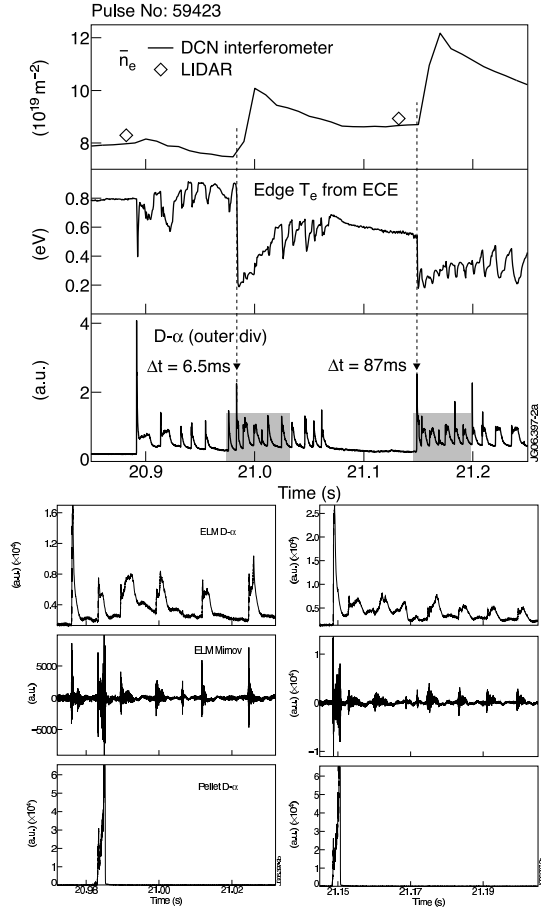
Figure 2: Pellets triggering ELMs at arbitrary times in the ELM cycle. Two pellets triggering ELMs despite different elapsed time since previous event. Hatched sequences on expanded time scale below.
