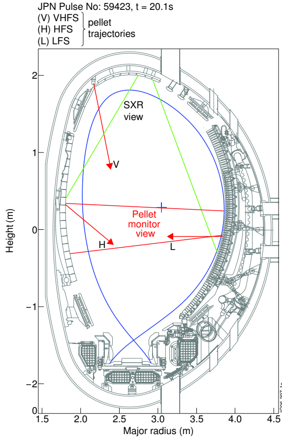
Figure 1: Poloidal cross section of JET tokamak with a typically used plasma separatrix contour, the three designated pellet injection tracks, observation areas covered by SXR camera and pellet ablation monitor.
