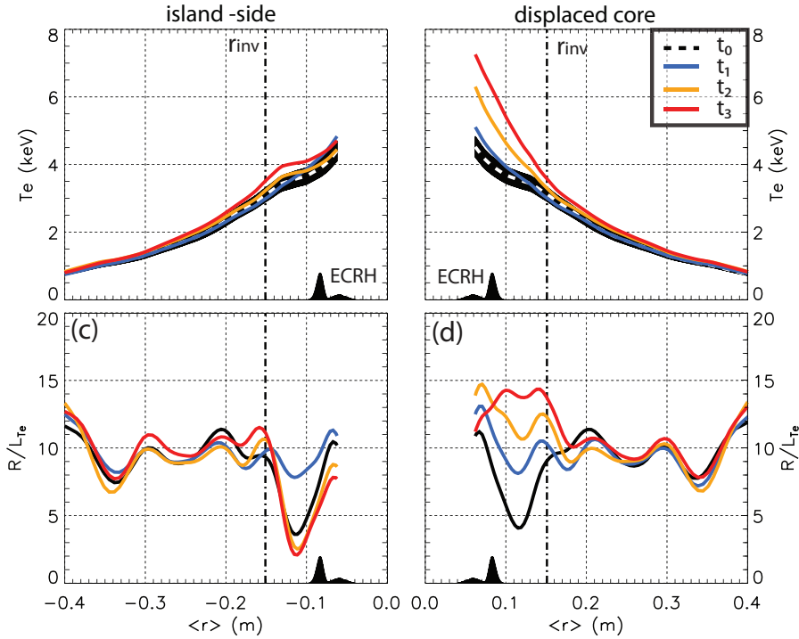
Figure 12. Electron temperature profiles on the island-side (a) and displaced core side (b) and their normalized logarithmic gradients, (c) and (d) respectively, for the time-points defined in figure 10. The black band of the T_e profiles for t_0 show the error on the electron temperature profiles.
