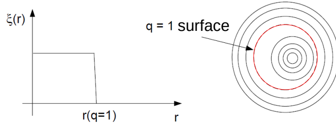
Figure 2.7: q=1 kink mode.
