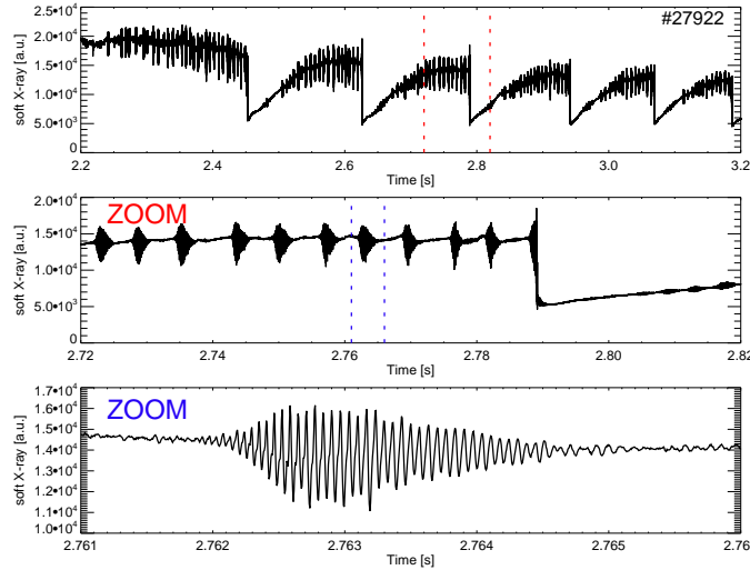
Figure 2.8: Soft X-ray measurement of fishbone modes and sawtooth crashes in ASDEX Upgrade. In the top row, the sawtooth crashes become visible. In the bottom row, which shows a zoom on one single fishbone instability, the fluctuation imposed by this kink mode can be seen.
