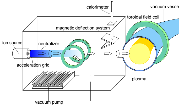
Figure 2.1: Scheme of neutral beam injection. The ions created in the so called ion source are first accelerated in the acceleration grid and then neutralized. Then, they are injected into the plasma.
