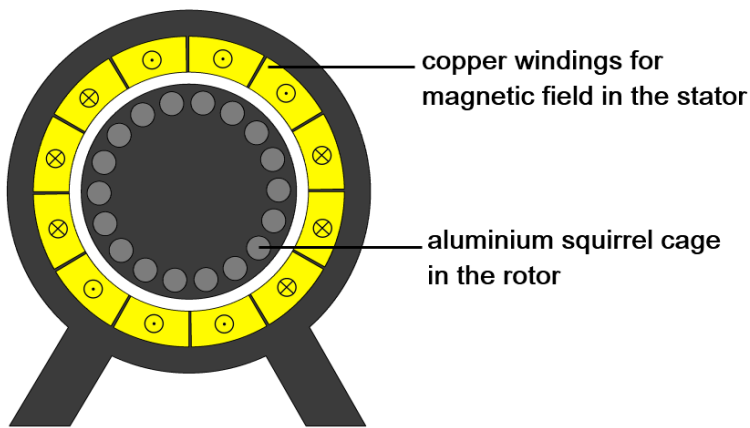
b) Asynchronous, or induction motor
