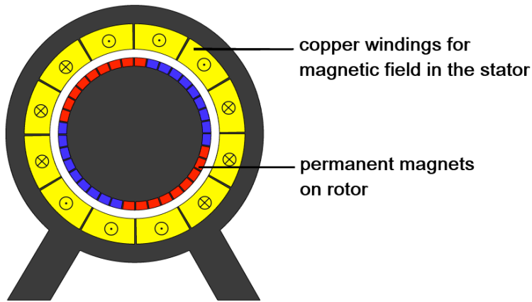
a) Permanent magnet synchronous motor
