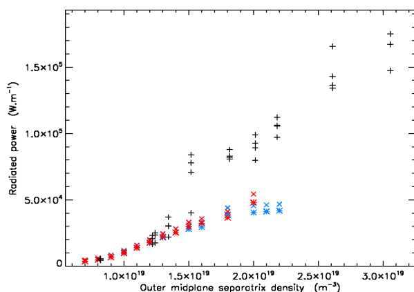
Figure 6. Measured and cumulative simulated powers radiated from the divertor. + measured, * D and x D+D 2 +D 2 + lines. Power to SOL 2.2 MW blue symbols and 2.8 MW red.
