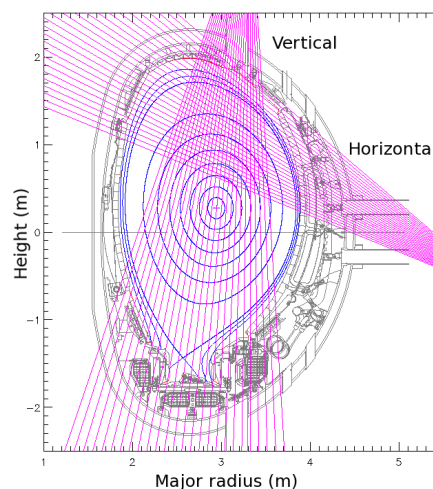
Figure 1. The spectrometer lines-of-sight.
