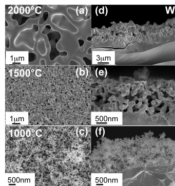
FIG. 8. Evolution of the helium-induced surface morphology changes of tungsten surfaces as a function of the surface temperature during plasma exposure ( E_{ion}=45 eV). For each temperature, top-views and cross-sections are shown on the left and right sides, respectively. The exposure duration was 1000 s for the samples prepared at 1500°C and 2000°C, and 500 s for the sample prepared at 1000°C.
