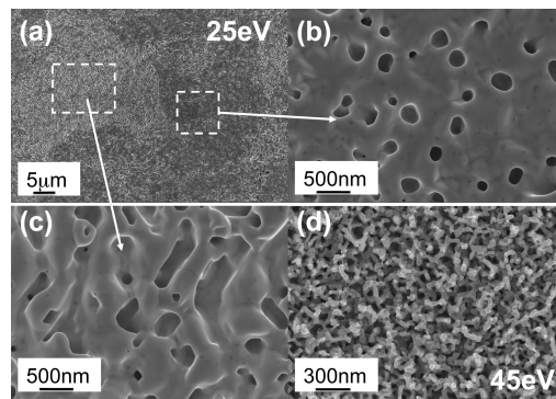
FIG. 3. Surface morphology of molybdenum surfaces induced by helium plasma exposure for a duration of 500 s, with a surface temperature of 1000^{\circ}\text{C} as a function of the impinging ion energy.
