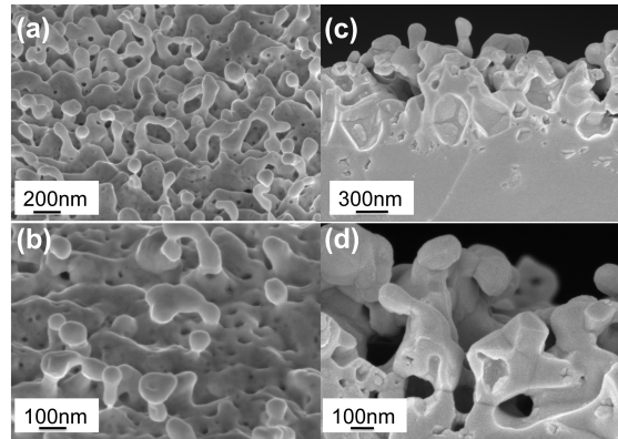
FIG. 5. Scanning electron microscope images of tungsten surface after exposure to a helium fluence of 3 \times 10^{26} m^{-2} (500 s) with a surface temperature of 1400^\circ C , with E_{ion} = 25 eV (a and b- with a tilt of 45^\circ ) and E_{ion} = 45 eV (c and d- cross-section images)
