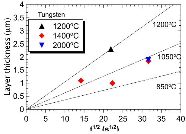
FIG. 9. (Color online) Evolution of the thickness of the nanostructured region as a function of exposure time for tungsten surfaces, with E_{ion}=45 eV.
