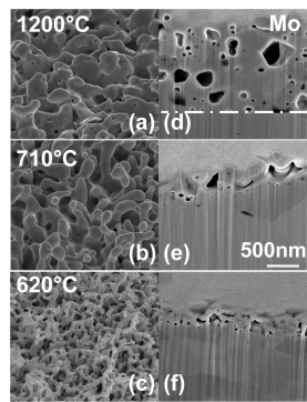
FIG. 6. Evolution of the helium-induced surface morphology changes of molybdenum surfaces as a function of the surface temperature during plasma exposure ( E_{ion}=45 eV, t=1000 s). For each exposure temperature, top-views (tilted by 52^\circ ) and cross-sections are shown in the same magnification on the left and right sides, respectively.
