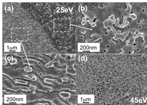
FIG. 4. Surface morphology of tungsten surfaces induced by helium plasma exposure for a duration of 500 s, with a surface temperature of 1000°C as a function of the impinging ion energy.
