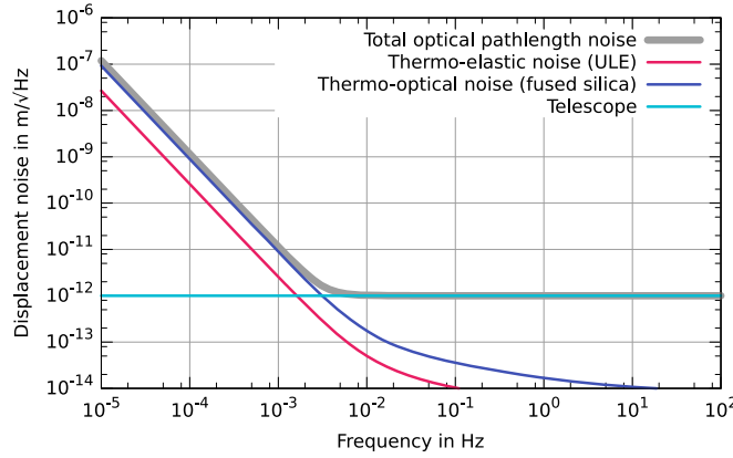
Figure 13. Total optical path length noise and individual contributions from the optical bench and telescope. The summation of the contributions is described in equation (39).
