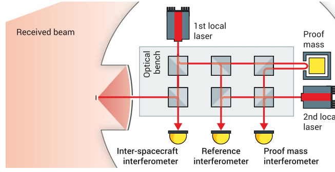
Figure 5. The measurement of the proper distance between any two proof masses is split into individual interferometers. Here, at each end of the link there are three interferometers, one to read out the inter-spacecraft distance, one to determine the displacement of the local proof mass in relation to the optical bench, and one acting as a reference.
