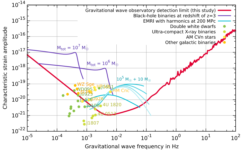
Figure 19. Observatory detection limit (for SNR = 1) and dimensionless characteristic strain amplitudes for different gravitational wave sources. Two traces for systems of binary black holes at redshift of z = 3 (total mass M_{\text{tot}} = 10^7 M_{\odot} and = 10^6 M_{\odot} ), where the former trace starts at low frequencies \approx 1 month, the latter \approx 1 year before the plunge (spike in the trace). First five harmonics of one eccentric extreme mass ratio inspiral (EMRI) for an object with mass m = 10 M_{\odot} captured by a massive black hole of mass M = 10^5 M_{\odot} at 200 Mpc distance. The EMRI trace starts at low frequencies many years before the merger. A selection of known ultra-compact binary stars (dots) for 1 year of observation time.
