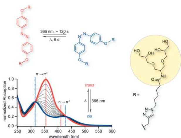
Fig. 1 UV/VIS absorption spectra showing the trans to cis conversion of G1azoG1 6 . The photoinduced isomerization is completed after 120 s, whereas the thermal cis to trans conversion takes 6 d when stored in the dark. The side chains of G1azoG1 6 are abbreviated by an "R".
