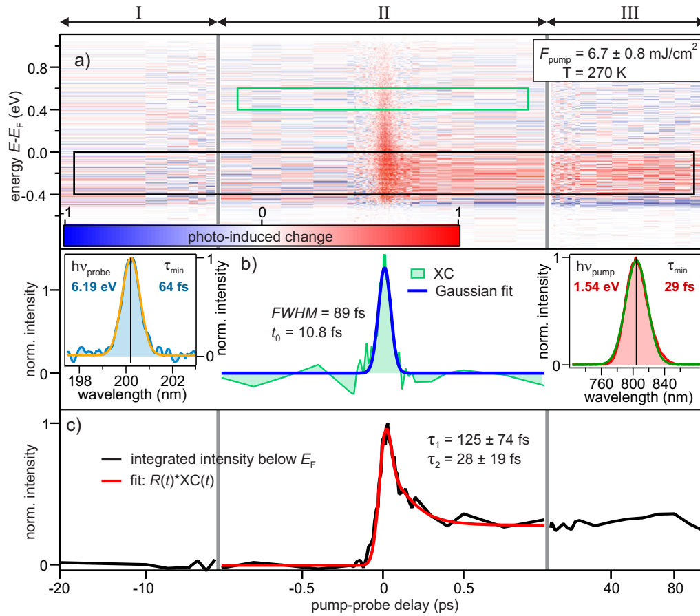
Figure 4.27: Overview over exemplary time-resolved PES dataset: a) shows the change in photoemission intensity induced by a F = 7 \text{ mJ/cm}^2 pump pulse, centred at 1.54 \text{ eV} photon energy, when probed by UV ( h\nu = 6.19 \text{ eV} ) light. Region I ( < -1 \text{ ps} ) has been used for background subtraction of the uncorrelated signal. The XC of the employed laser pulses (green) taken from the region indicated by the green box and a Gaussian fit (blue) are displayed in b). The insets show laser spectra of probe (left) and pump (right) light. The transient evolution of DOS below the Fermi energy (region indicated by black box in a)) is shown in c). The fit with an empirical model (response R(\Delta t) convolved with cross correlation from b)) yields the red curve.
