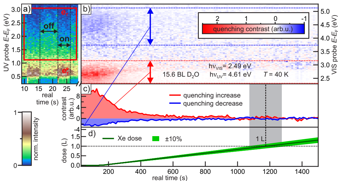
Figure 6.4: Xenon overlayer on top of ASW/CU(111). Intensity changes in photoemission upon UV plus VIS illumination (on) in contrast to UV-only illumination (off) are shown in a). The quenching contrast (on minus off) is shown in b) with respect to real time and energy upon xenon adsorption. Integrated increase and decrease (region of integration is indicated by the arrows) are shown in c). d) Shows the adsorbed amount of xenon.
