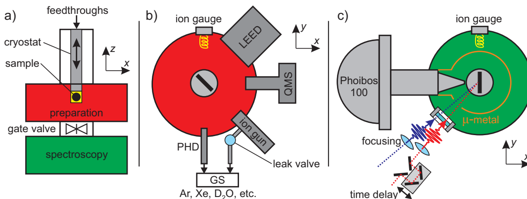
Figure B.1: UHV chamber: a) Sample is fixed on cryostat and can be moved (along x , y , z ) and rotated (around z ). UHV chamber for preparation (red) is separated from spectroscopy chamber (green) by a gate valve. Overview of preparation chamber is shown in b): LEED and QMS for characterisation, ion gun for single crystal surface preparation, PHD for D_2O adsorbate dosing. The spectrometer part is displayed in c): Phoibos 100 electron analyser and incoupling window for focused laser pulses. Time delay control via linear translation stage is indicated. See text for details.
