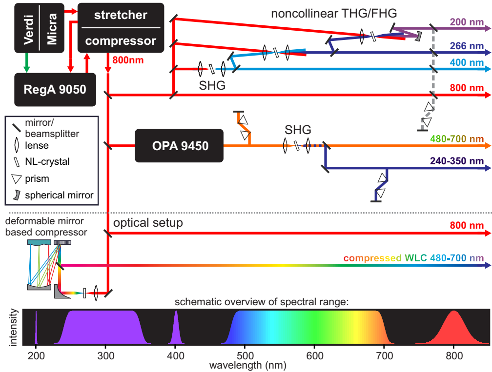
Figure 3.1: Schematic overview of the optical setup: The commercial Coherent laser system involving CW-pump-laser ( Verdi ), femtosecond oscillator ( Micra ), regenerative amplifier ( RegA 9050 ) and collinear optical parametric amplifier ( OPA 9450 ) generates ultrashort laser pulses tunable over the visible spectral range. This range is extended into the UV by exploiting nonlinear optical effects, yielding a widely tunable light source. Achievable photon energies are depicted schematically at the bottom of the figure. For the all-optical experiments the fundamental 800 nm pulses as well as adaptively compressed WLC pulses, spanning the whole visible wavelength range, are used.
