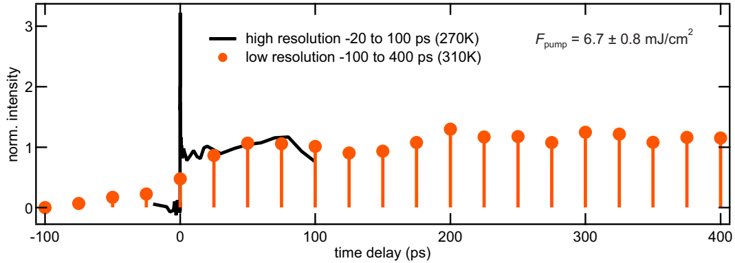
Figure 4.34: Transient change of DOS below the Fermi energy (interval of between -0.4 and 0 eV with respect to E_F ) up to 400 ps: A low time resolution scan up to pump-probe delays of 400 ps (orange) is shown for an incident excitation fluence of 6.7 \pm 0.8 \text{ mJ/cm}^2 . Data with better time resolution (black) from Figure 4.27 c) is displayed for comparison. Both datasets have been normalised to an average between 20 and 100 ps.
