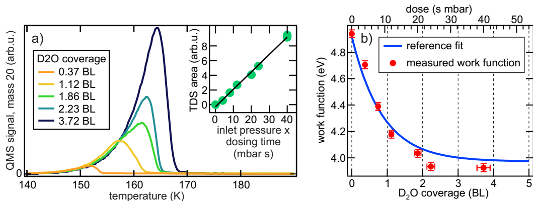
Figure 6.1: Characterisation of amorphous D 2 O-layers via TPD and work function: in a) TPD spectra for various D 2 O-coverages are displayed. The inset confirms the linear relation between inlet pressure times dosing time and integrated TPD intensity. In b) a reference fit (blue) performed in [Dei11] is used to translate dose into coverage in BL, via the measured change in work function (red) of the system.
