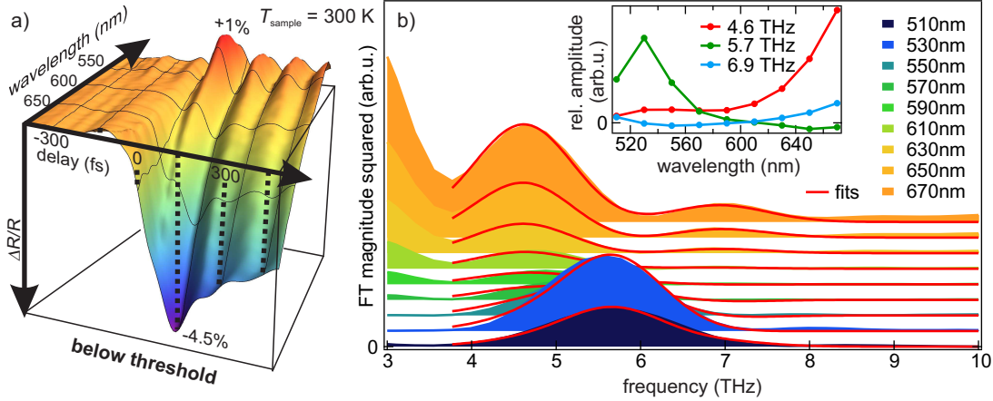
Figure 4.5: a) Broadband reflectivity change upon pump excitation at room temperature and below phase transition threshold fluence. b) FFTs of lineouts at indicated wavelengths of a) ( \pm 10 nm) and Gaussian fits to three detected phonon oscillations (curves are offset for clarity). Relative phonon amplitude with respect to probe wavelength is shown in the inset. Mind the opposite ordering of wavelengths in a) and b).
