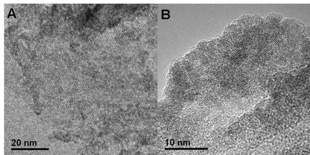
Fig. 2 HR-TEM images of \text{KCl/SnCl}_2 -derived carbon nitride composite showing (A) lattice fringes of the carbon nitride sheets with the distance of \sim 1.0 nm and (B) \text{SnO}_2 NPs.
