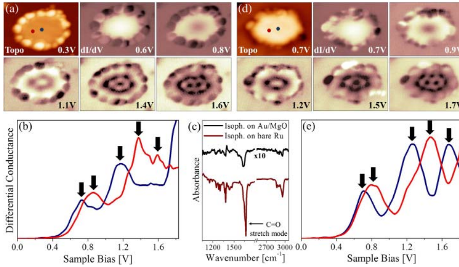
FIG. 2 (color online). Topographic and dI/dV maps of an Au island (a) with and (d) without isophorone molecules bound to its perimeter ( 11 \times 8 \text{ nm}^2 , 70 \text{ pA} ). (b) and (e) associated conductance spectra taken in the center (blue) and the left part of the island (red) as indicated in (a) and (d). Gaussian fitting revealed five QWSs that are marked by arrows. Their bias positions match the ones used for dI/dV imaging in (a) and (d). (c) Infrared absorbance spectra of isophorone adsorbed on Au/MgO (black) and Ru(0001) (gray). Similar vibrational modes are resolved in both cases, indicating that the molecule adsorbs associatively on the two surfaces.
