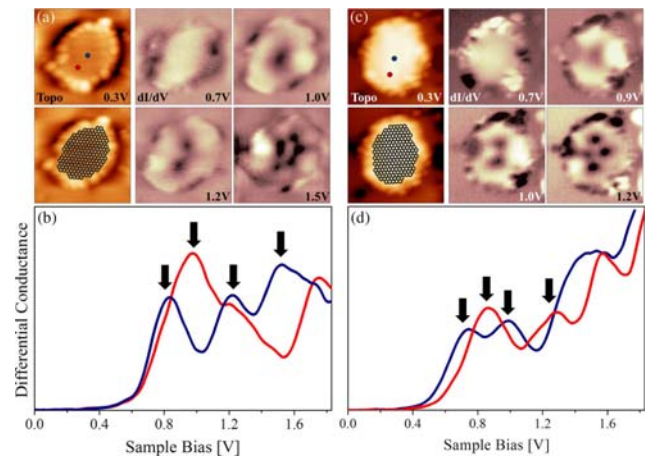
FIG. 3 (color online). Topographic and dI/dV images of an Au island (a) with and (c) without \text{CO}_2 molecules bound to its perimeter ( 8 \times 8 \text{ nm}^2 , 70 \text{ pA} ). Associated dI/dV spectra taken in the island center (blue) and slightly below (red) are shown in (b) and (d). The arrows depict the positions of four QWSs revealed from Gaussian fitting. The respective bias values match the ones used for dI/dV imaging in (a) and (c).
