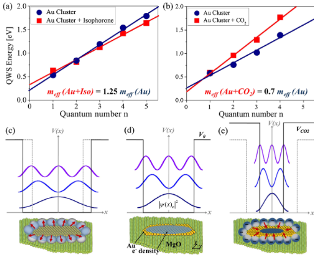
FIG. 4 (color online). Dispersion relation of QWSs in Au islands with/without (a) isophorone and (b) \text{CO}_2 . The modified E(n) slope can be translated into different effective electron masses that become larger in presence of isophorone but smaller after \text{CO}_2 adsorption. 1D scheme showing the electron confinement in (c) an Au island with isophorone, (d) a pristine island and (e) an island with edge-bound \text{CO}_2 . Attractive isophorone-Au forces promote electron spill-out in (c), which increases the potential well and causes the QWSs to move together. Conversely, charge transfer into the \text{CO}_2 generates a repulsive rim around the island that results in a compression of the Au electron gas and moves the QWSs apart (e).
