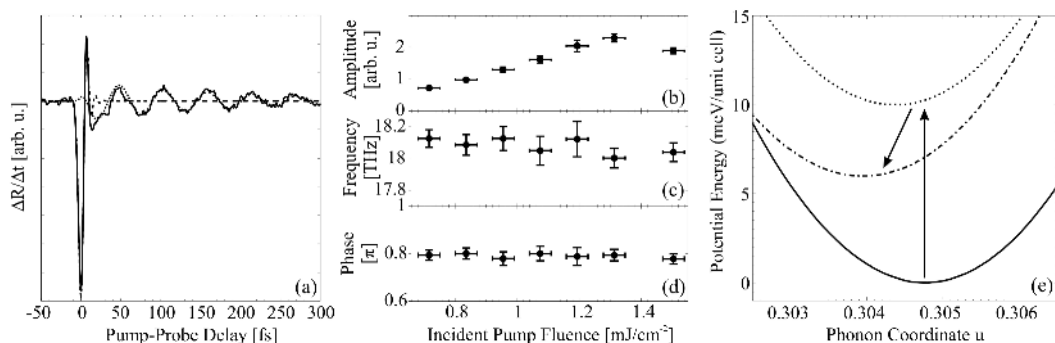
Fig. 1. (a) Differential UV reflectivity change as a function of pump-probe delay (solid line) and fit consisting of two components: The initial, rapid dynamics leading to the overall drop in reflectivity (dashed line) and the coherent phonon oscillation (dotted line). The amplitude (b), frequency (c), and oscillation phase shift (d) are shown as a function of incident pump fluence. (e) Calculations of the potential energy surfaces (PES) of the A_1 phonon in \text{TiO}_2 : ground state (solid line), 1 eV-hot excited state (dotted line), and cold excited state (dash-dotted line) PES. The curves were shifted vertically for presentation purposes.
