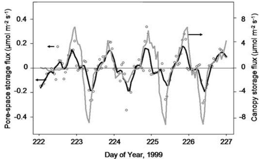
Fig. 8. Below-ground pore-space CO 2 storage flux (data points and 3-h running average, black curve) and below-canopy CO 2 storage flux (3-h running average, grey curve).
