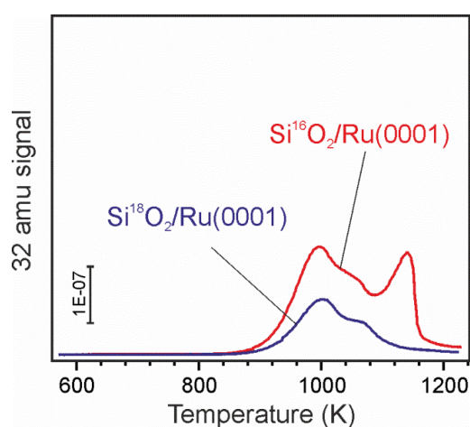
Figure 3. Oxygen (32 amu) signal in TPD spectra of SiO 2 /Ru(0001) films prepared with 16 O and 18 O isotopes as indicated. Both films were then exposed to 15 mbar 16 O 2 at 700 K for 45 min. Note that the 18 O-labeled film additionally contained silica nanoparticles (see Fig. S2 in Supporting Information).
