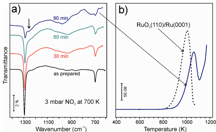
Figure 4. (a) IRA-spectra of SiO 2 /Ru(0001) after stepwise exposure to 3 mbar NO 2 at 700 K for the total time as indicated. Total exposure time is indicated. The arrow on panel (a) highlights the feature commonly assigned to three-dimensional silica particles caused by film dewetting. Oxygen TPD spectrum taken for the last sample is shown in (b). Spectrum for RuO 2 (110)/Ru(0001) from Fig. 1a is shown as dashed line, for comparison
