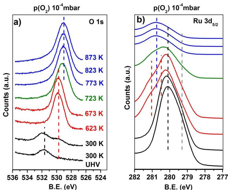
Figure 6. O 1s (a) and Ru 3d 5/2 (b) regions in AP-XPS spectra taken in 10 -4 mbar of O 2 at increasing temperatures as indicated. The lowermost spectra are obtained in UHV for the clean Ru(0001) surface prior to the oxygen exposure. The photon energy is 580 eV. The spectra are offset for clarity.
