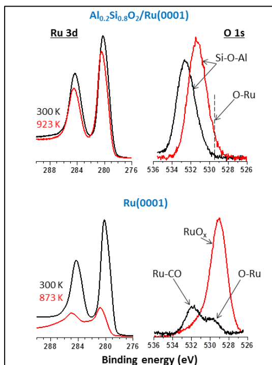
Figure 7. Ru 3d and O 1s regions in XP-spectra of the bare Ru(0001) surface and the aluminosilicate film measured at 300 K and after heating in 10^{-4} mbar \text{O}_2 to the indicated temperatures.
