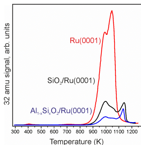
Figure 5. Comparative TPD spectra of O 2 (32 amu) from three different samples as indicated. All were exposed to 15 mbar of O 2 at 700 K for 40 min.
