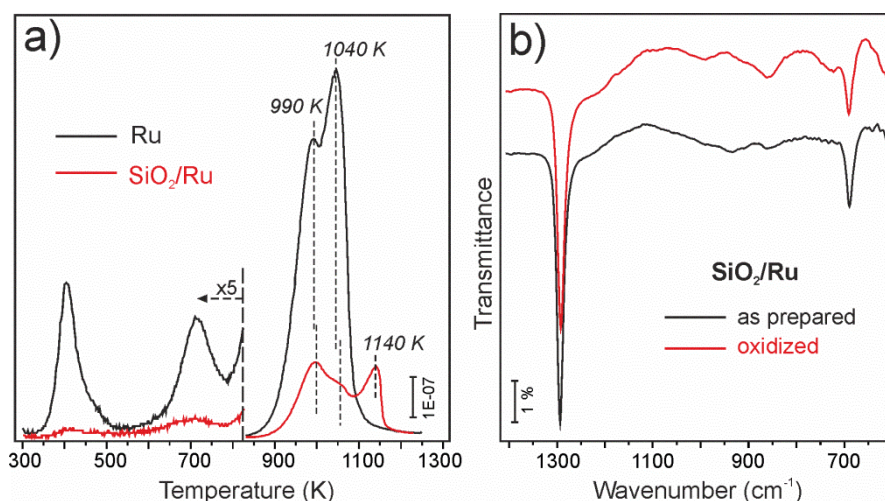
Figure 2. (a) O 2 (32 amu) signals in TPD spectra of Ru(0001) (in black) and SiO 2 /Ru(0001) (in red) surfaces after exposure to 15 mbar O 2 at 700 K for 45 min. (b) IRA-spectra of the SiO 2 /Ru(0001) film before (in black) and after (in red) oxygen exposure show that the structure of the silicate film is maintained.
