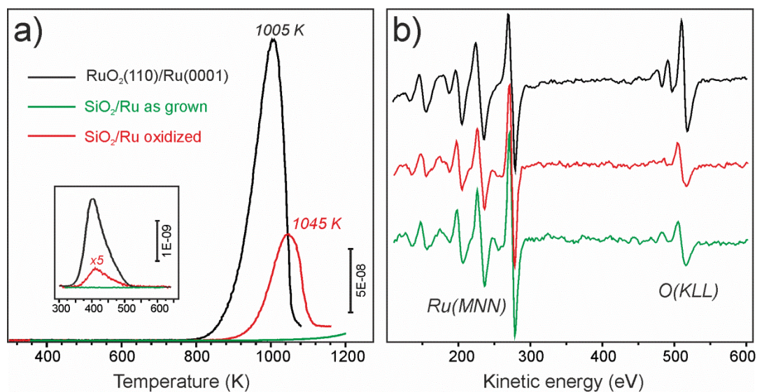
Figure 1. O 2 -TPD spectra (a) and AES spectra (b) of Ru(0001) (in black) and SiO 2 /Ru(0001) (in red) surfaces after exposure to 10 -5 mbar O 2 at 700 K for 45 min. The results for “as grown” SiO 2 /Ru(0001) (in green) are shown for comparison.
