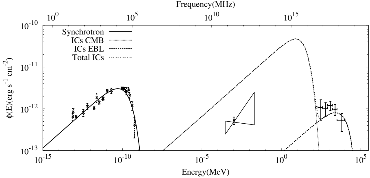
Figure 9. The broadband SED of Fornax A for Model I, where both the X-rays and \gamma -rays are produced by IC scattering by the synchrotron-emitting electrons. The IC scattering contribution from the EBL and the CMB photon fields are both shown in the figure. The model parameters are described in Table 2.
