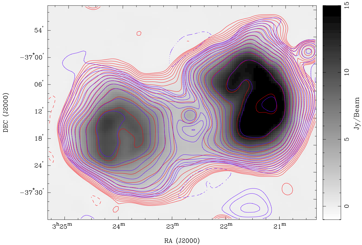
Figure 2. Fornax A at 154 MHz (gray scale and red contours) overlaid with the VLA 1.5 GHz (Fomalont et al. 1989) contours, after smoothing to the MWA resolution, in blue. Positive contours are solid and increment in a geometric progression of \sqrt{2} , starting at 0.1 Jy/beam for the 154 MHz image and 0.05 Jy/beam for the 1.5 GHz image. The broken red contour is at -0.1 Jy/beam and the broken blue contour is at -0.05 Jy/beam.
