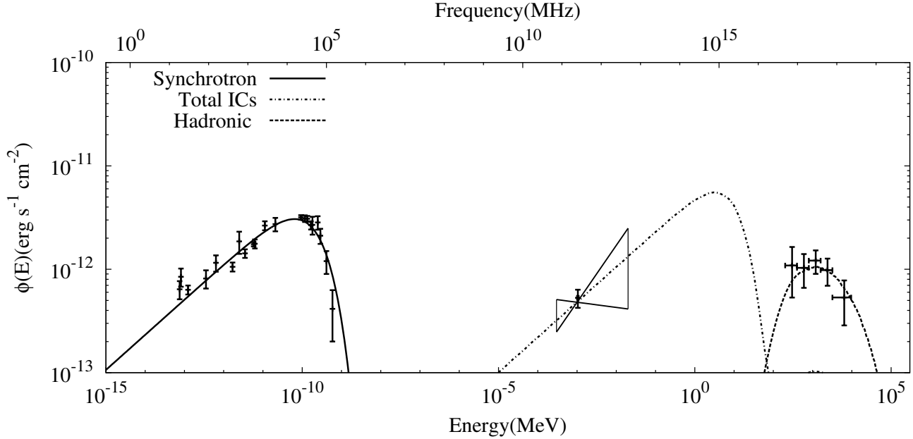
Figure 11. The broadband SED of Fornax A for Model III, where the X-ray emission is the result of IC scattering by the synchrotron-emitting electrons and the \gamma -rays are produced by p-p collisions with pion decay. The model parameters are described in Table 2.
