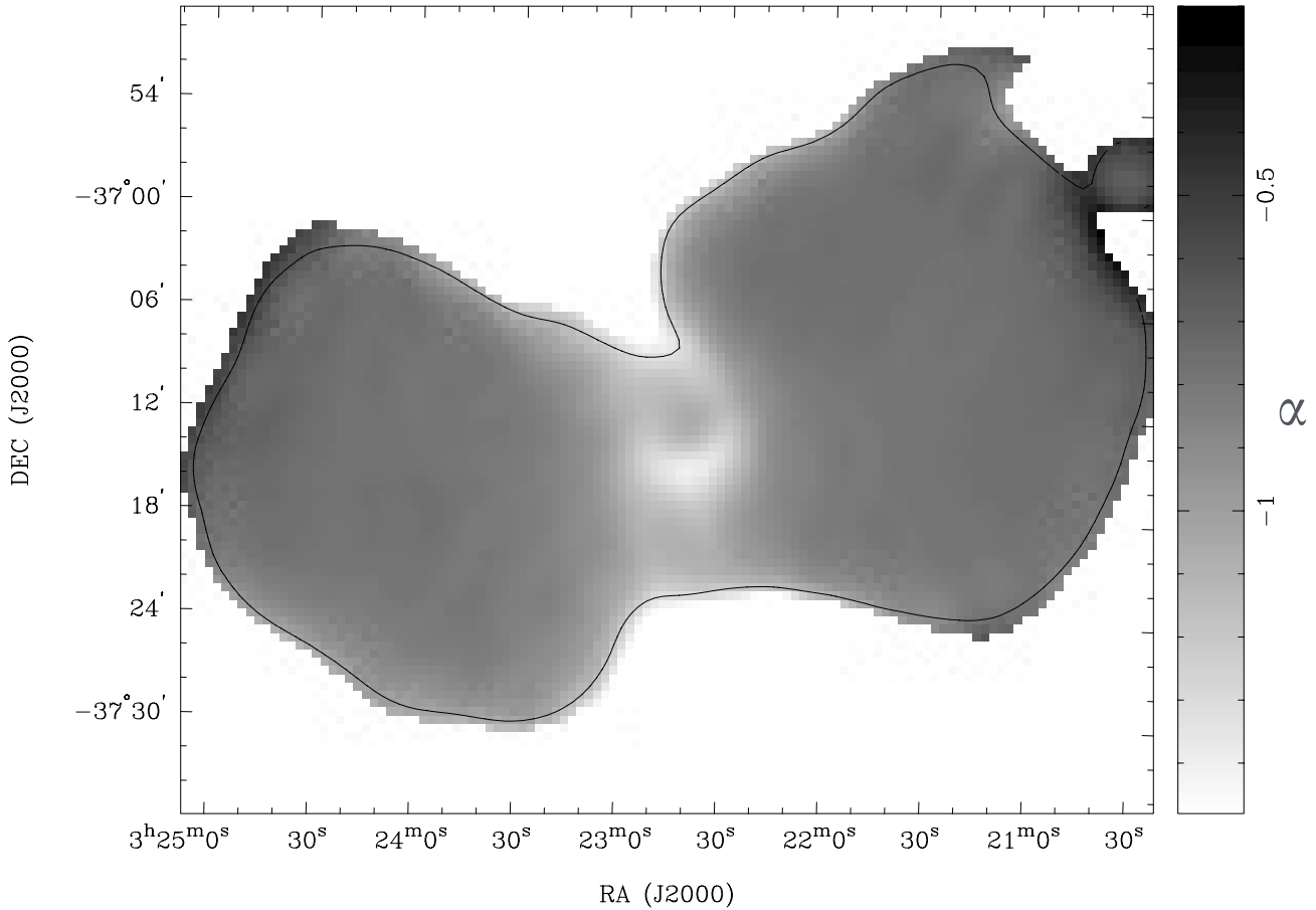
Figure 7. Spectral index map of Fornax A. The contour shown is the 0.1 Jy/beam level from the smoothed VLA image at 1510 MHz. White pixels outside of the contour are blanked and there are no blanked pixels inside the contour. The map shows that the spectral index varies only slightly across the lobes, from the average value of approximately -0.77 , but that the bridge region has a significantly steeper spectrum; reaching a value of -1.4 just to the south of the core.
