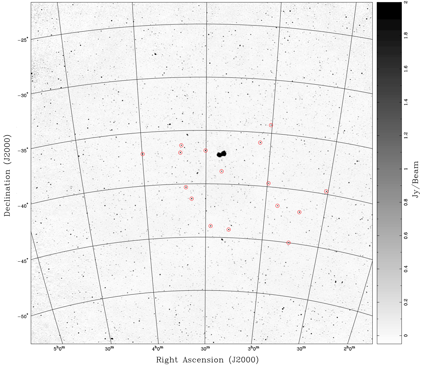
Figure 1. Fornax A and surrounding field at 154 MHz with the Murchison Widefield Array. The image is shown on a linear scale between -0.05 and +2 Jy/beam. It has an angular resolution of 185 arcsec and an rms noise of approximately 15 mJy/beam in ‘empty’ regions of the image more than 1^\circ away from Fornax A. The red circles mark the positions of the Culgoora sources (Slee 1977, 1995) used to set the flux-density scale.
