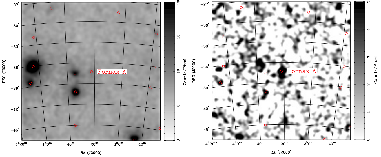
Figure 3. \gamma -ray counts image (left panel) and residual image (right panel) above 100 MeV in the ROI. The sources in the 2FGL catalogue are marked as red circles.
