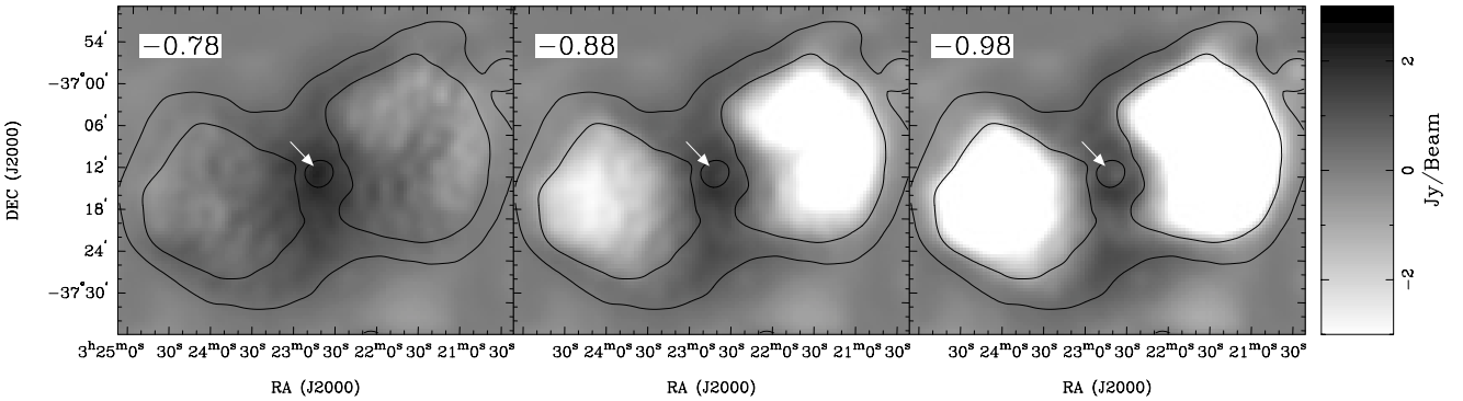
Figure 6. As for figure 6, but with trial spectral indices between -0.78 and -0.98 . The unresolved core of Fornax A, indicated by the white arrow, has a flatter spectrum than the surrounding diffuse bridge emission.
