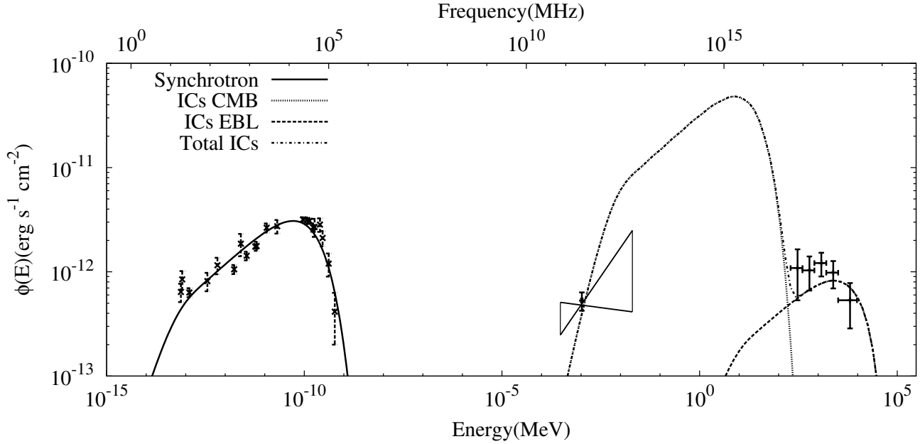
Figure 10. The broadband SED of Fornax A for Model II, where both the X-rays and \gamma -rays are produced by IC scattering by the synchrotron-emitting electrons, which are described by an electron energy distribution with a low-energy cut-off. The model parameters are described in Table 2.
