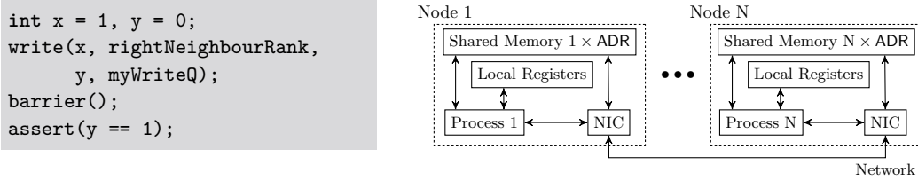
■ Figure 1 (a) Program 1to1 is the compute and exchange results idiom often found in PGAS applications. Each process copies an integer value to its neighbour. write asks the hardware to copy the value of address x to y on the right neighbouring node. barrier blocks until all processes reach the barrier. The assertion can fail, as the barrier may execute before the write completes. (b) PGAS architecture — NIC stands for network interface controller.
