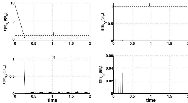
FIGURE 4. Example 2: Average values (over 100 experiments) of the distance of the solution process \xi_{x_0 v} to the sets W (left panels) and Z (right panels), in two different vertical scales (top vs bottom panels).
