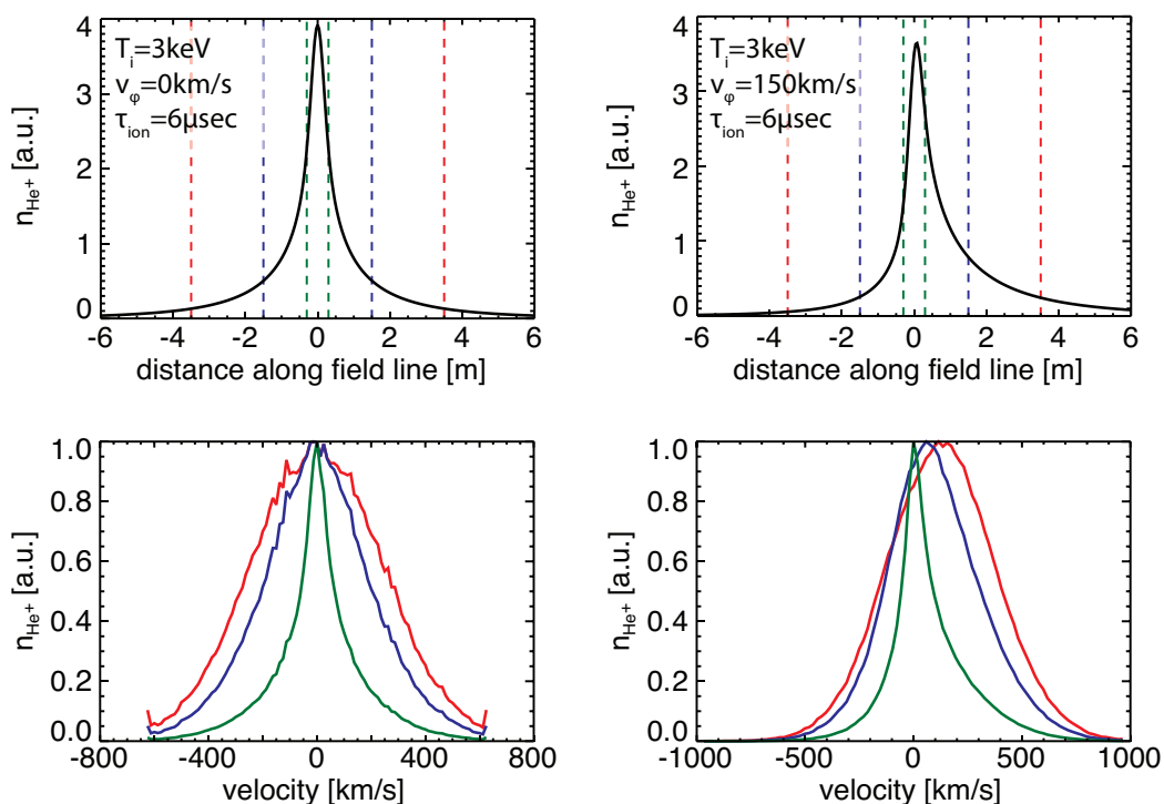
Figure 5.4: Distribution of plume ions along a magnetic field line (top plots) for zero rotation (left) or v_\phi = 150 \text{ km/s} (right). In the bottom, the corresponding velocity distributions of plume ions summed over the ranges indicated in the top plots.
