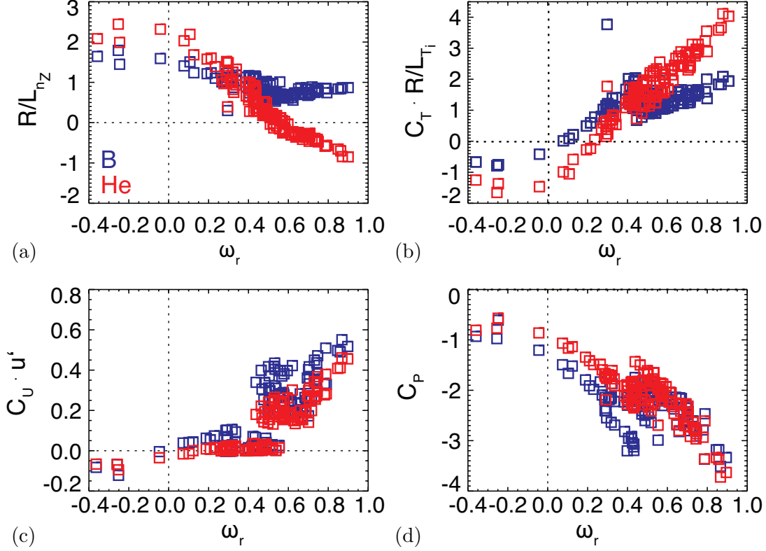
Figure 6.11: Predicted R/L_{nB} and R/L_{nHe} (a) and turbulent contributions to the impurity transport, namely (b) the thermodiffusive term, (c) rotodiffusive term and (d) the pure convection term for each impurity at \rho_{tor} = 0.5 .
