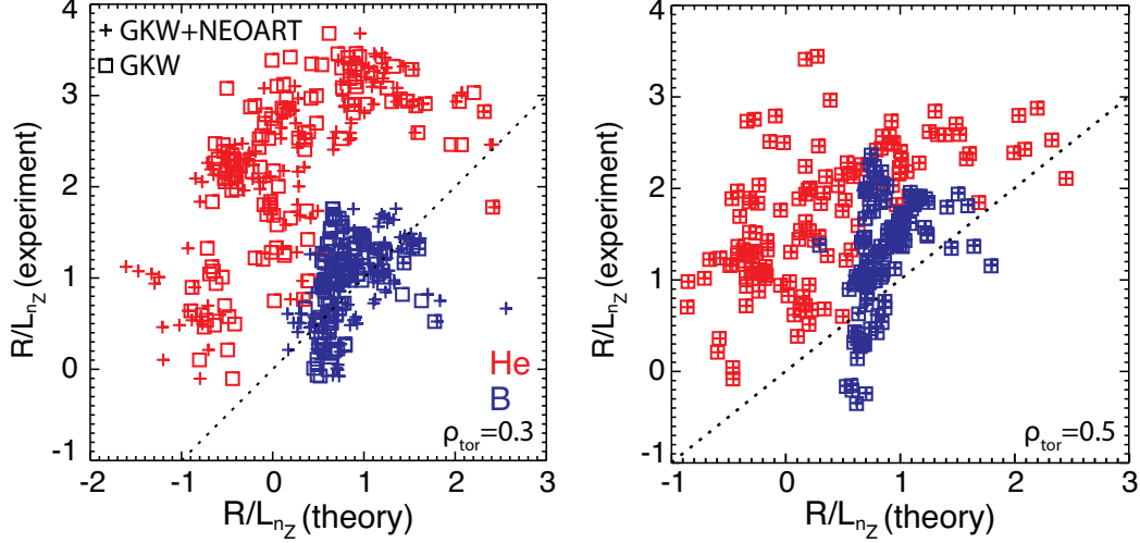
Figure 6.14: R/L_{n_{He}} and R/L_{n_B} deduced from the experiment in comparison to the theoretical predictions at \rho_{tor} = 0.3 and \rho_{tor} = 0.5 , from GKW (only turbulent transport, squares) and from GKW and NEOART (both neoclassical and turbulent transport, crosses).
