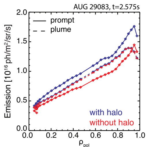
Figure 5.12: The effect of including the neutral beam halo in the modelling of the prompt and the plume emission.
