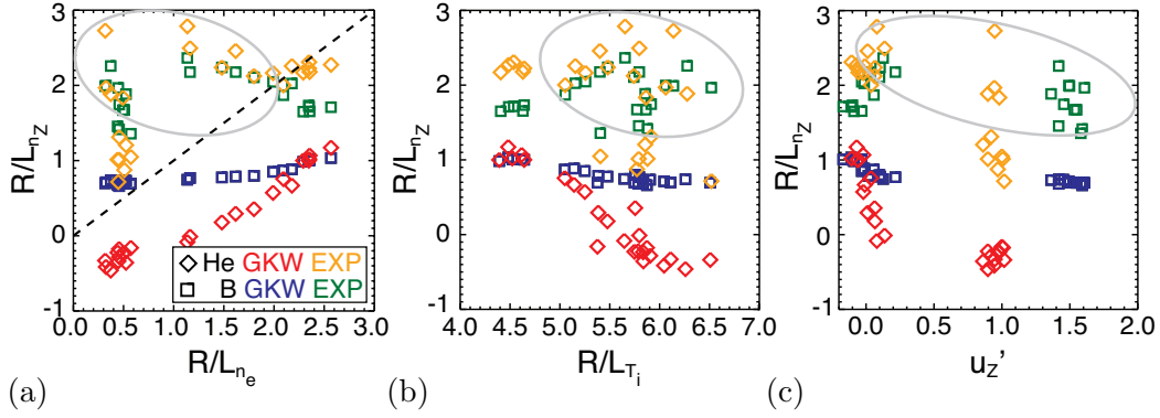
Figure 6.18: R/L_{n_{He}} and R/L_{n_B} , both from gyrokinetic modelling predictions and experimental measurements \rho_{tor} = 0.5 , plotted against a) R/L_{n_e} , b) R/L_{T_i} and c) u'_z , for discharge 30380. The circles highlight the odd points.
