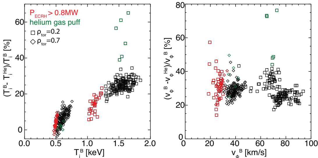
Figure 5.19: Comparison of toroidal rotation and ion temperatures at \rho_{tor} = 0.2 and \rho_{tor} = 0.7 derived from helium and boron charge exchange measurements for all measurement time points in discharge 29083. Time points with additional ECRH power or close to a helium puff are indicated.
