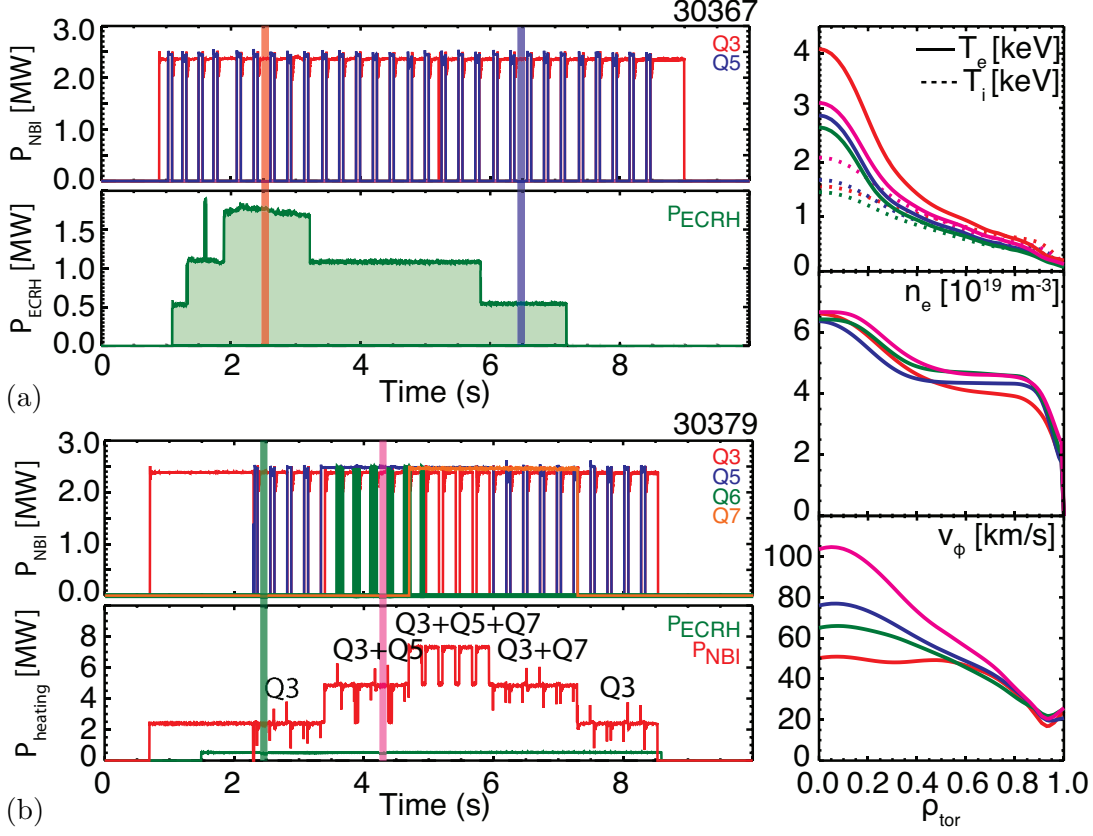
Figure 6.1: Heating schemes of two discharges from the helium transport database. a) In discharge 30367, a scan of ECRH power at constant NBI power was performed, in order to vary the peaking of the electron density profile. b) In discharge 30379, a scan of NBI power at constant ECRH power was performed, in order to see the effect of on- and off-axis beams and NBI power levels on the impurity density profiles.
