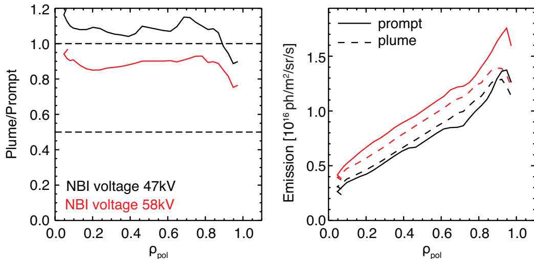
Figure 5.11: The plume-to-prompt emission ratio as well as the prompt and plume emissions are compared for two different neutral beam injection voltages, 58kV and 47kV, which are within the operational range of the ASDEX Upgrade neutral beam injection systems, including the full, half and third energy components and the beam halo.
