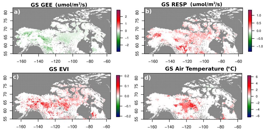
Figure 8. Sen's slope of median change (2001–2012) in PolarVPRM estimates of growing season carbon cycle variables, and driver data. All statistically significant ( p value < 0.05) changes over time in carbon cycle variables and driver data are shown for the growing season (GS, when SCA < 50 % AND GEE < 0). Please note that as the growing season includes only the period of time for which vegetation is productive at any pixel (GEE < 0), periods of time for which air temperature extremes or drought hinder photosynthesis are not included. The influences of rising EVI and air temperatures on increasing Arctic rates of photosynthesis are therefore made clear, whereas plots of annual GEE (Fig. 7) emphasize reductions in photosynthetic uptake of C by forest vegetation.
