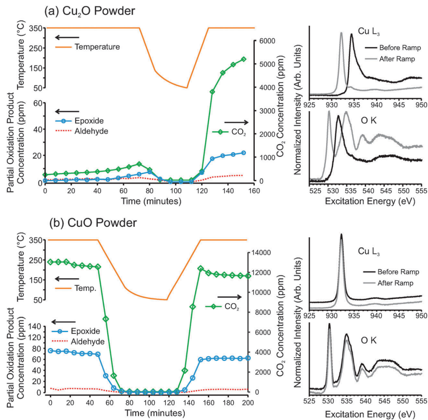
Fig. 6 (left) Gas chromatography product analysis and (right) in situ measured NEXAFS spectra of (a) \text{Cu}_2\text{O} and (b) \text{CuO} powders heated in a 1:1 mixture of \text{O}_2 and \text{C}_2\text{H}_4 at 0.3 mbar.
