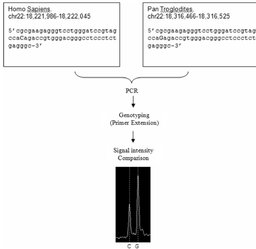
Figure 1. Schematic representation of the principle of quantitative interspecies competitive PCR. Human and P. troglodytes specific alleles are represented by alleles 'C' and 'G', respectively.
