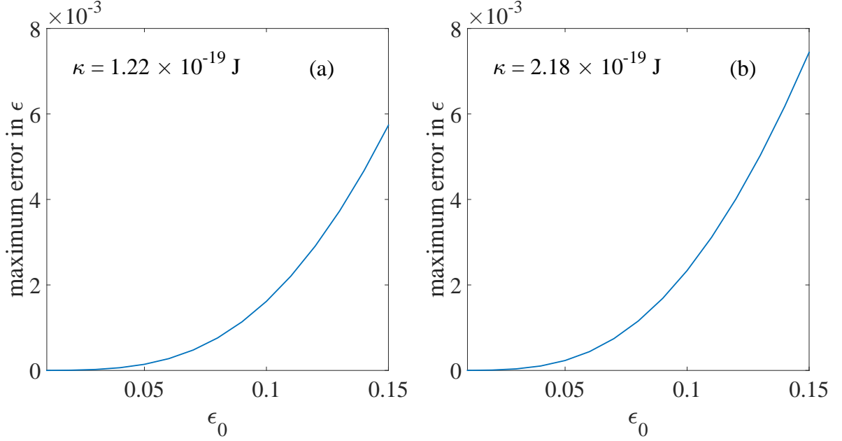
FIG. S2: Maximum error of \epsilon between numerical solutions to Eq. (1) and Eq. (4), plotted as a function of \epsilon_0 . (a) \kappa = 1.22 \times 10^{-19} \text{ J} (POPC). (b) \kappa = 2.18 \times 10^{-19} \text{ J} (POPC with 30% cholesterol).
