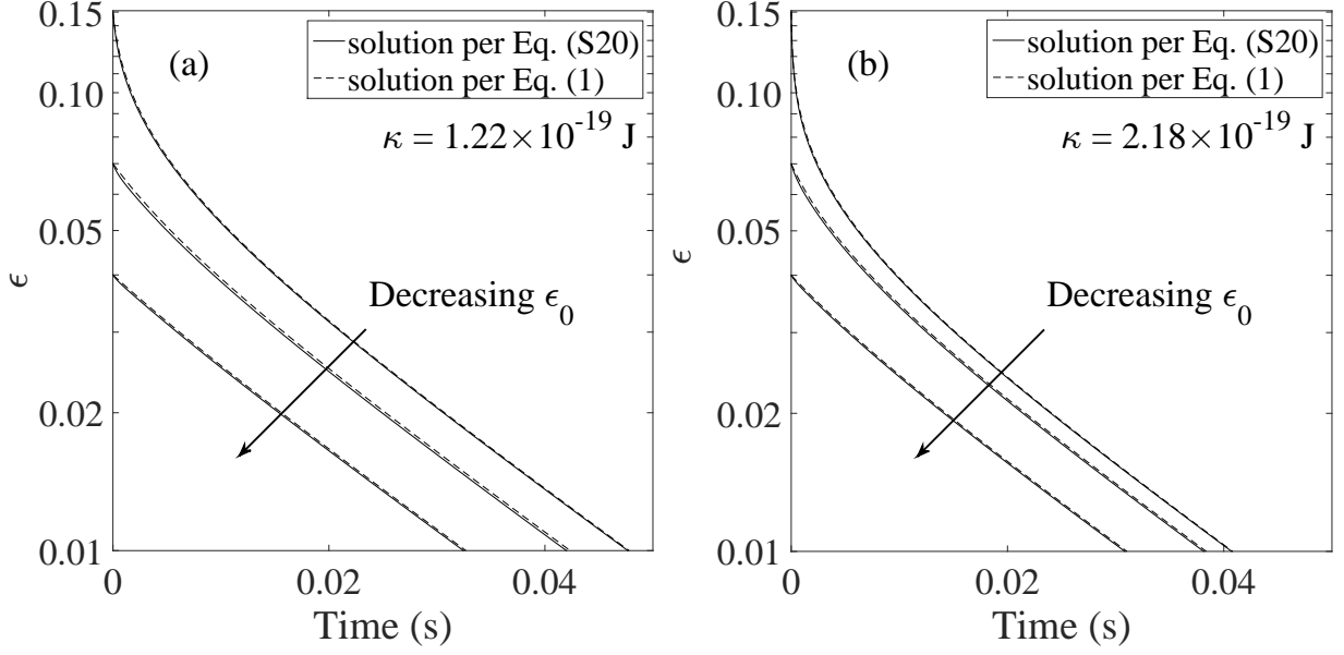
FIG. S3: Comparison between numerical solutions to Eq. (S20) (with discharging effect) and Eq. (1) (without discharging effect), for \epsilon_0 = 0.04, 0.07 and 0.15 , respectively. (a) \kappa = 1.22 \times 10^{-19} J (POPC). (b) \kappa = 2.18 \times 10^{-19} J (POPC with 30% cholesterol). In both figures, the strengths and the lengths of the applied electric pulses are (50\text{V}, 50 \mu\text{s}) , (50\text{V}, 100 \mu\text{s}) , and (80\text{V}, 100 \mu\text{s}) , corresponding to \epsilon_0 = 0.04, 0.07 , and 0.15 , respectively. These protocols are chosen as they typically resulted in similar values of \epsilon_0 in our experiments.
