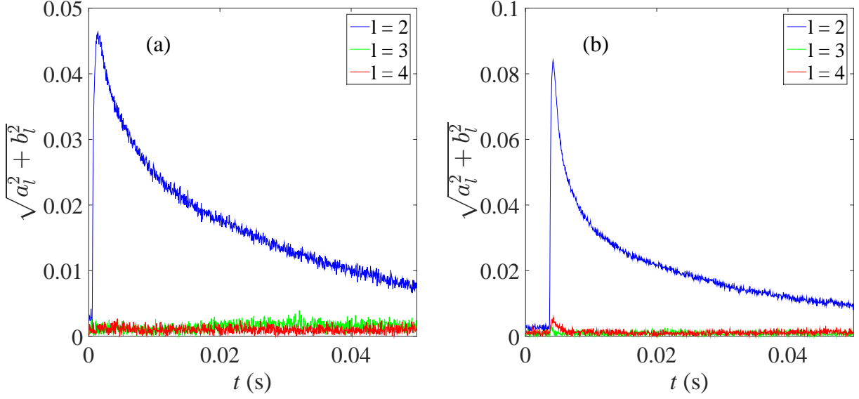
FIG. S4: Exemplary amplitude evolution of l = 2, 3 and 4 modes during relaxation. (a) Vesicle #4, POPC with 30% cholesterol (Table S5). (b) Vesicle #7, POPC (Table S2).
