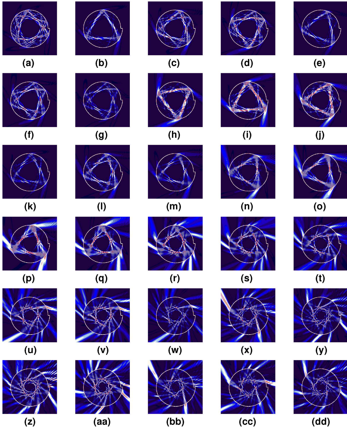
Figure 6. (Color online) Resonance patterns for n = 2 case. These correspond to the solid circles in Fig. 5, and are arranged in the increasing order of |\text{Im}(nkR)| . (The intensity of the fields is normalized by scaling the maximum intensity inside the cavity as one.) The calculated resonance positions are (a) nkR = (110.25, -0.0637) , (b) (110.54, -0.0871) , (c) (109.81, -0.0873) , (d) (109.88, -0.0887) , (e) (109.97, -0.0896) , (f) (110.89, -0.1003) , (g) (110.81, -0.1029) , (h) (109.70, -0.1128) , (i) (110.40, -0.1142) , (j) (110.09, -0.1174) , (k) (110.61, -0.1233) , (l) (109.76, -0.1367) , (m) (109.63, -0.1866) , (n) (110.12, -0.2198) , (o) (109.95, -0.2297) , (p) (110.65, -0.2543) , (q) (110.26, -0.2740) , (r) (110.31, -0.3078) , (s) (110.41, -0.3208) , (t) (109.55, -0.3375) , (u) (109.70, -0.3680) , (v) (109.80, -0.3684) , (w) (109.59, -0.3904) , (x) (110.01, -0.3927) , (y) (110.80, -0.3992) , (z) (110.91, -0.4002) , (aa) (110.70, -0.4036) , (bb) (110.11, -0.4063) , (cc) (109.92, -0.4066) , (dd) (110.59, -0.4164) , respectively.
