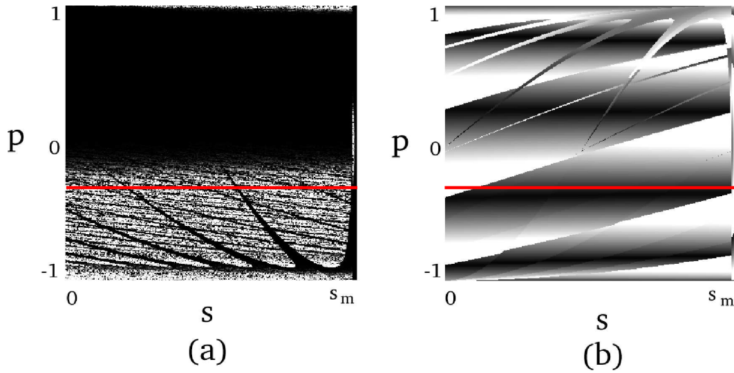
Figure 3. (a) The steady probability distributions P_s(s, p) , when n = 3 . (b) The distance distributions d_{m=5}(s, p) after five bounces. The similar distribution for n = 2 case is shown in Fig. 2 in [31]. From the comparison between P_s(s, p) and d_m(s, p) , it is clear that the partially reflected rays near p = -p_c (red line) make roughly (not exact) a triangle shape ( n = 2 ) and a star shape ( n = 3 ) trajectories.
