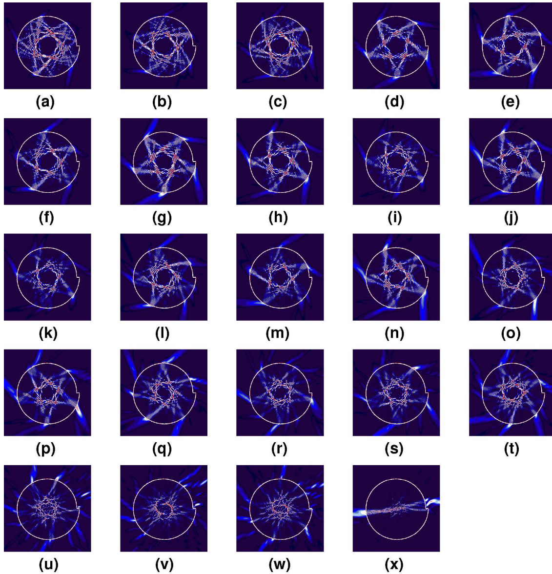
Figure 7. (Color online) Resonance patterns for n = 3 case. These correspond to the open triangles in Fig. 5, and are arranged in the increasing order of |\text{Im}(nkR)| . (The intensity of the fields is normalized by scaling the maximum intensity inside the cavity as one.) The calculated resonance positions are (a) nkR = (110.90, -0.0654) , (b) (109.92, -0.0766) , (c) (110.11, -0.0873) , (d) (109.60, -0.0907) , (e) (110.41, -0.0991) , (f) (109.78, -0.1030) , (g) (109.59, -0.1127) , (h) (110.68, -0.1135) , (i) (109.52, -0.1152) , (j) (110.63, -0.1303) , (k) (110.81, -0.1318) , (l) (110.33, -0.1330) , (m) (109.86, -0.1361) , (n) (110.56, -0.1403) , (o) (110.27, -0.1712) , (p) (110.95, -0.1718) , (q) (109.98, -0.1829) , (r) (110.12, -0.1855) , (s) (110.75, -0.1885) , (t) (109.73, -0.1920) , (u) (110.25, -0.2477) , (v) (110.87, -0.2491) , (w) (109.95, -0.2578) , (x) (110.65, -0.2962) , respectively.
