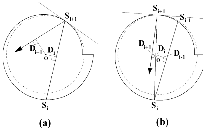
Figure 4. (a) The distance D_i always increases for counterclockwise propagating rays. (b) The clockwise propagating rays eventually change its direction of rotation as far as it does not hit the notch part. (The dotted line is a virtual circle passing i th bouncing point and having common origin with the spiral)
