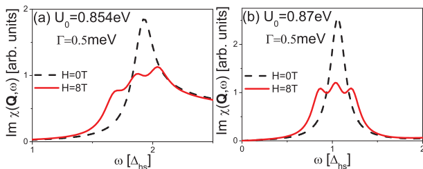
FIG. 3: (color online) \text{Im}\chi(\mathbf{Q}, \omega) for H = 0 \text{ T} (dashed black curve) and H = 8 \text{ T} (solid red curve) at T = 2 \text{ K} .
