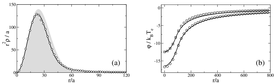
Figure 1. (a) Comparison of the electron density obtained from a full MD-simulation (circles) of 50000 ions and electrons with \Gamma_e(t=0) = 0.5 with the corresponding Michie-King distribution (solid line). The shaded area shows the ion density profile. (b) Numerically calculated electrostatic potential for N_i = 300000 , \Gamma_e = 0.2 (circles) and N_i = 300000 , \Gamma_e = 0.05 (squares), compared to the fit formula Eq.(4).
