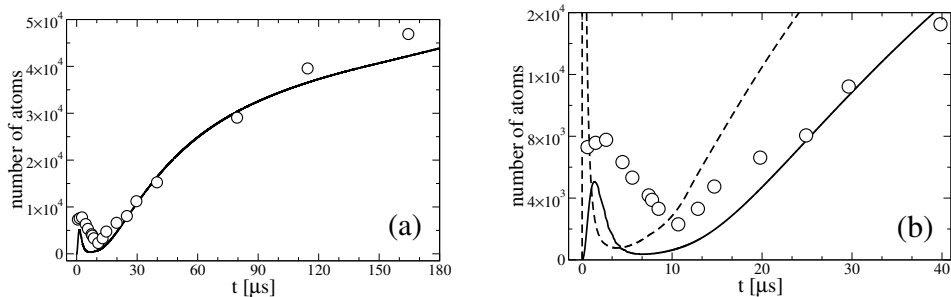
Figure 3. Comparison of the calculated (solid line) time dependence of the number of Rydberg atoms with the experiment [2] (circles) for N_i(t=0) = 700000 , \rho(t=0) = 2.7 \times 10^9 \text{cm}^{-3} and T_e(t=0) = 6\text{K} . The dashed line in (b) shows the result without the effect of ionic microfields (see text).
