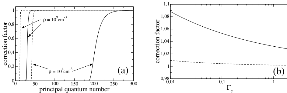
Figure 2. (a) Average correction factor for ionization rates (solid line) and n \rightarrow n+1 -excitation rates (dashed line) for N_i = 500000 and \Gamma_e = 0.2 at two different densities, as indicated by the arrows. (b) Average correction factor for recombination rates (solid line) and total deexcitation rates (dashed line) for N_i = 500000 .
